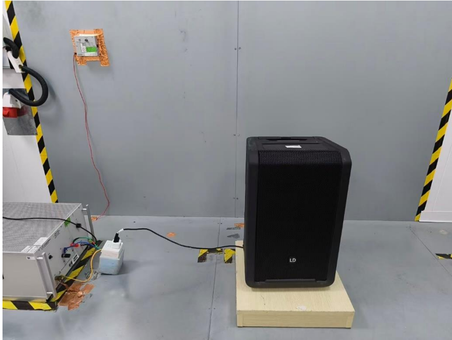
Set-up for Radio Spectrum
