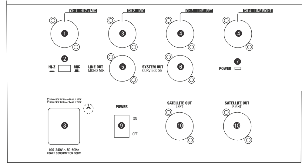
LDCURV500S
