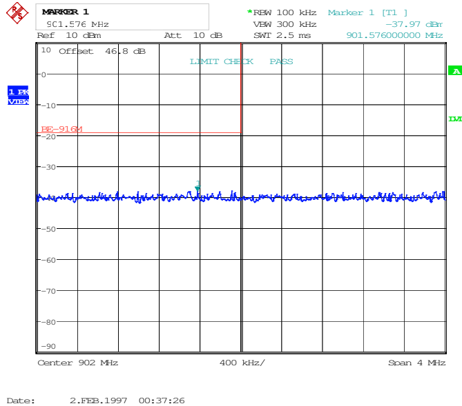
Figure 8.3-1: Bandedge Measurement, low
