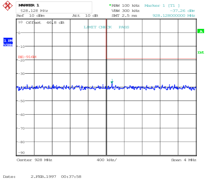
Figure 8.3-2: Bandedge Measurement, high
