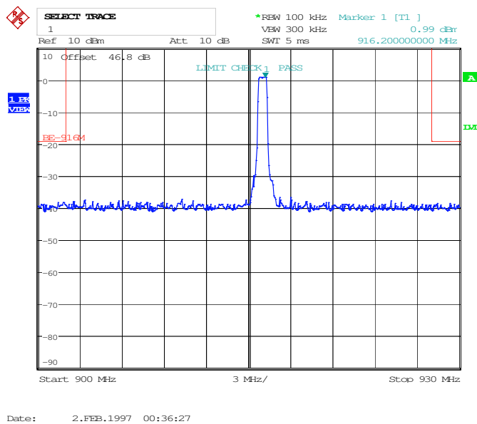
Figure 8.3-3: Bandedge Measurement, Overview
