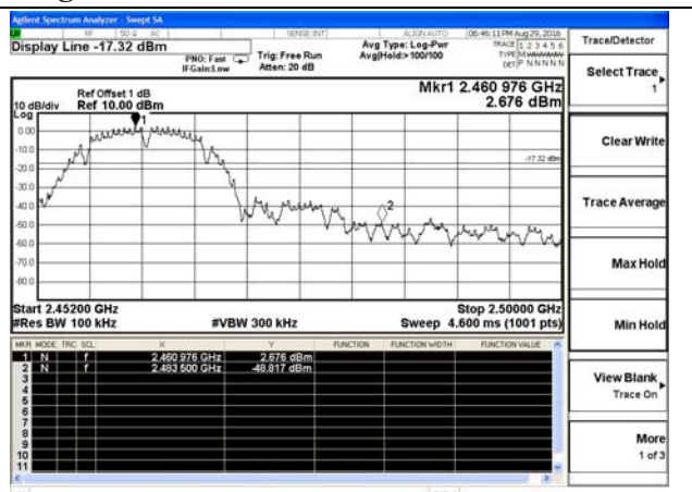
802.11b_High Channel / 2462MHz
