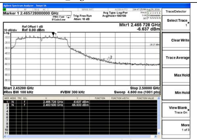
802.11g_High Channel / 2462MHz
