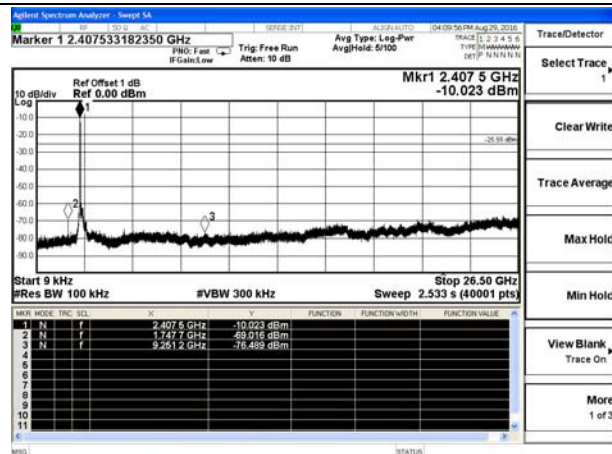
802.11n HT20_Low Channel / 2412MHz
