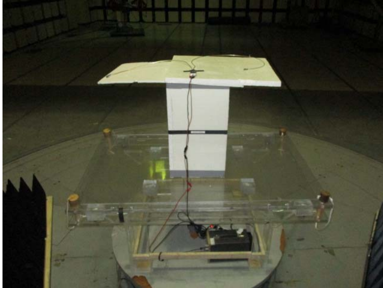
Radiated Measurements > 1 GHz, Front
