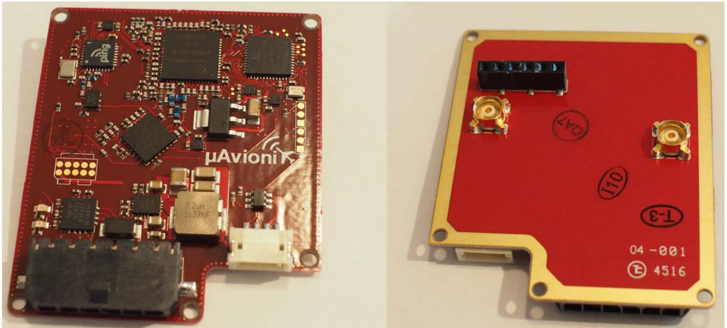
Logic/RF Board, Top and Bottom
