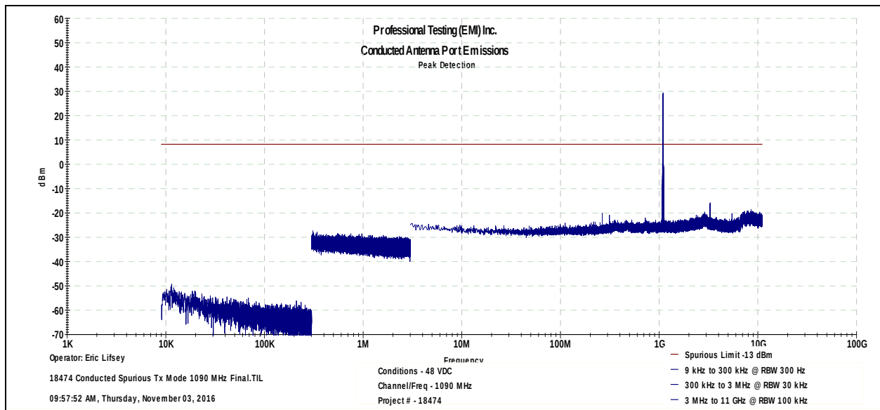
Conducted Antenna Port Spurious; Full Range 9 kHz to 11 GHz
