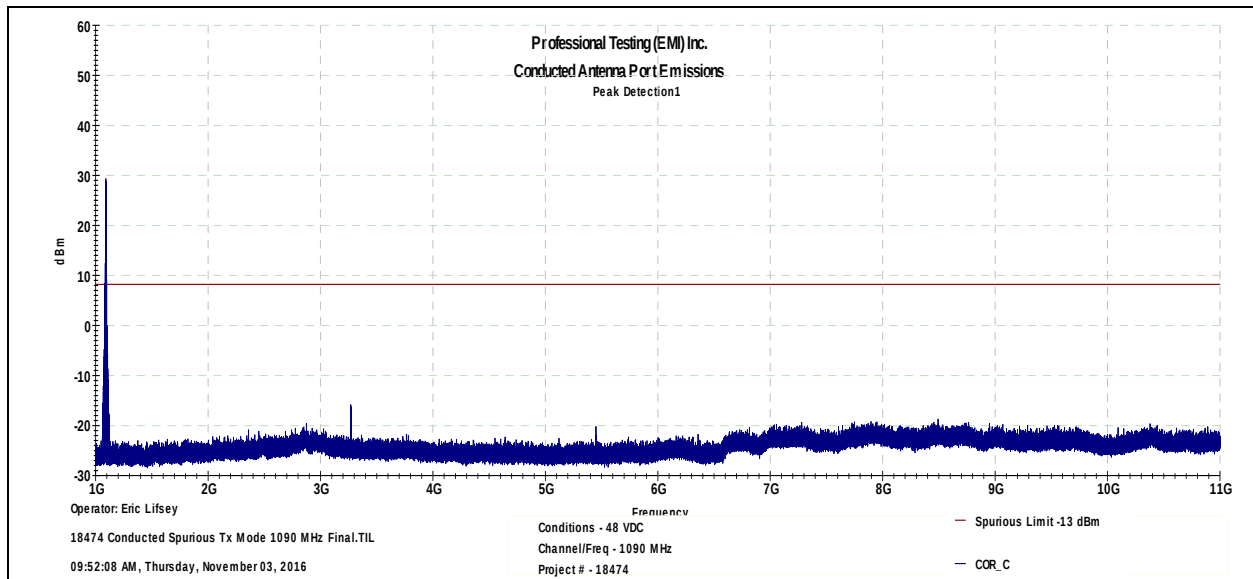
Conducted Antenna Port Spurious; Expanded for 1 GHz to 11 GHz
