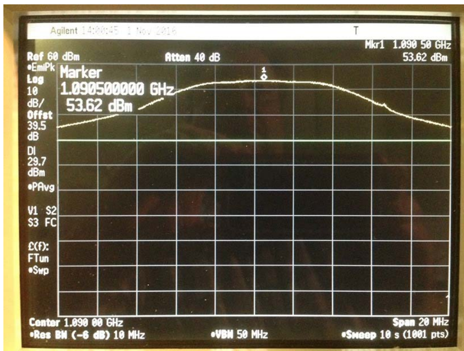
Peak Power
