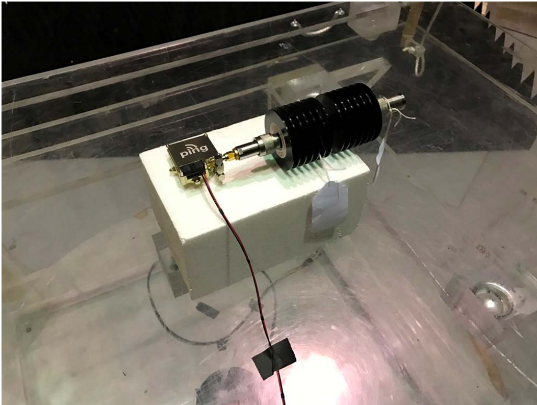
Spurious Emissions
