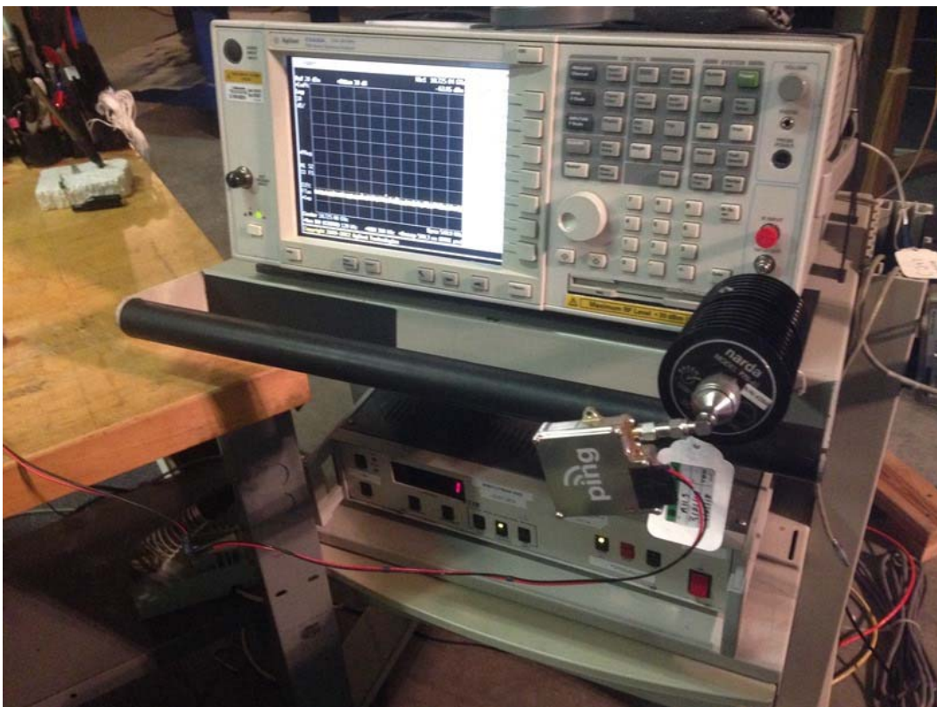
Conducted Port: Bandwidth, Power, Spurious, Modulation Characteristics
