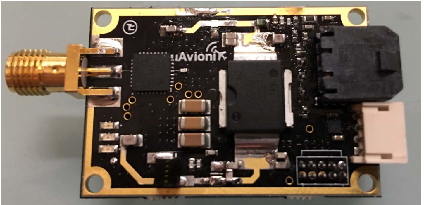
RF Board, Side 1
