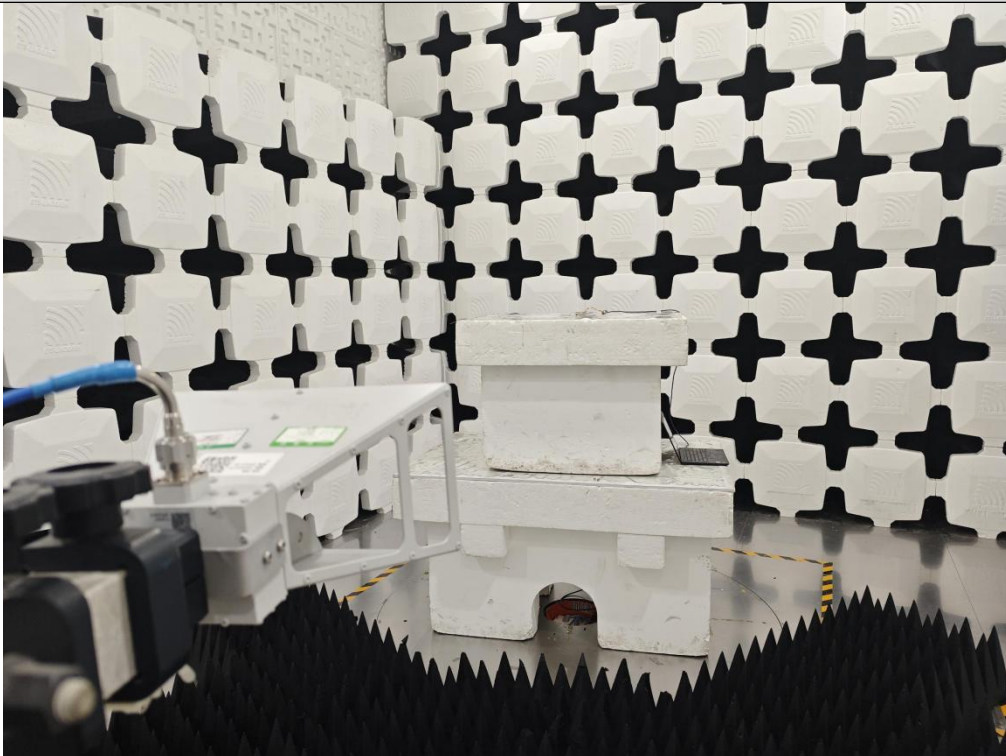
AC Power Line Conducted test
