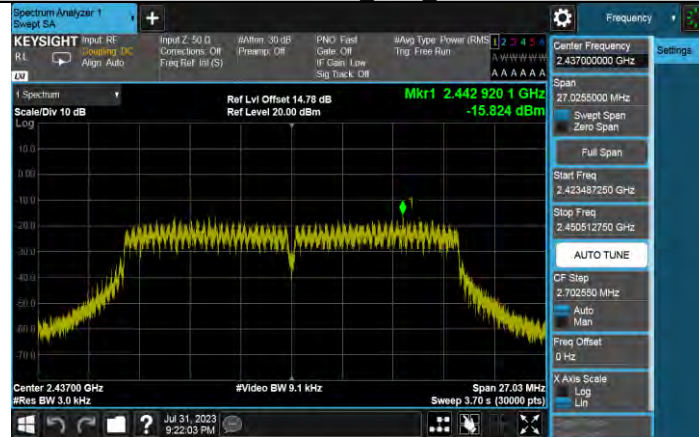
11N20SISO Ant2_2437
