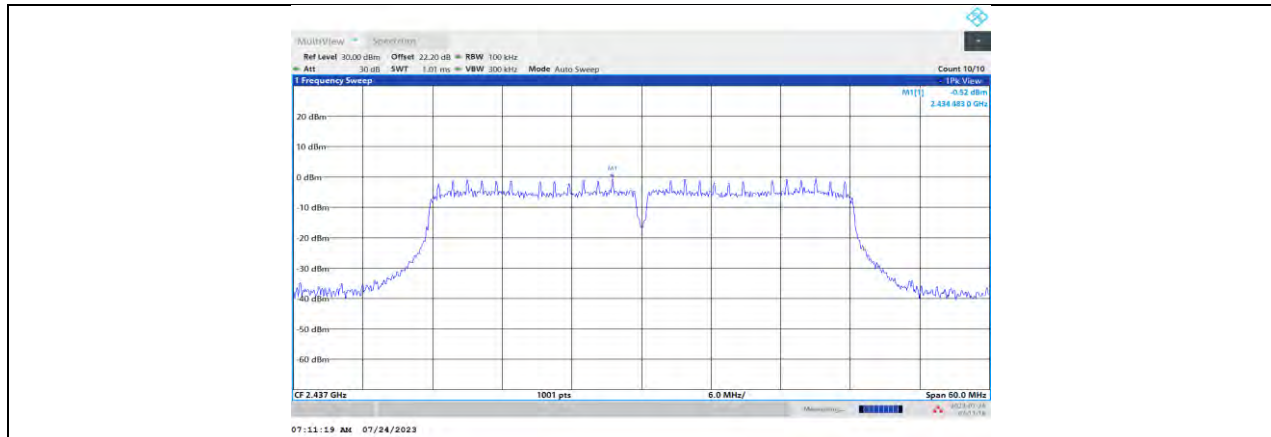
11N40SISO_Ant2_2437_0~Reference
