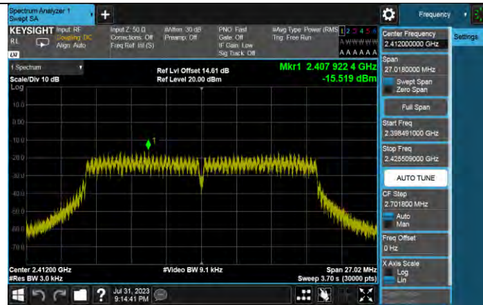
11N20SISO Ant2_2412
