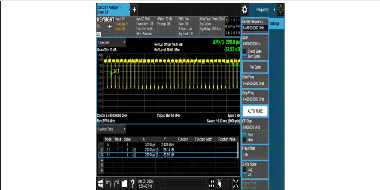
NTNV-11BE40MIMO-Ant1-6485
