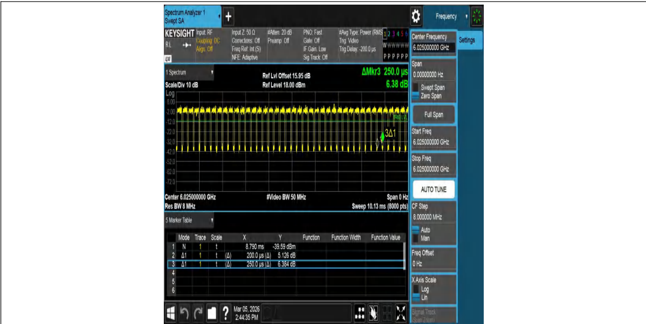
NTNV-11AX160MIMO-Ant1-6025
