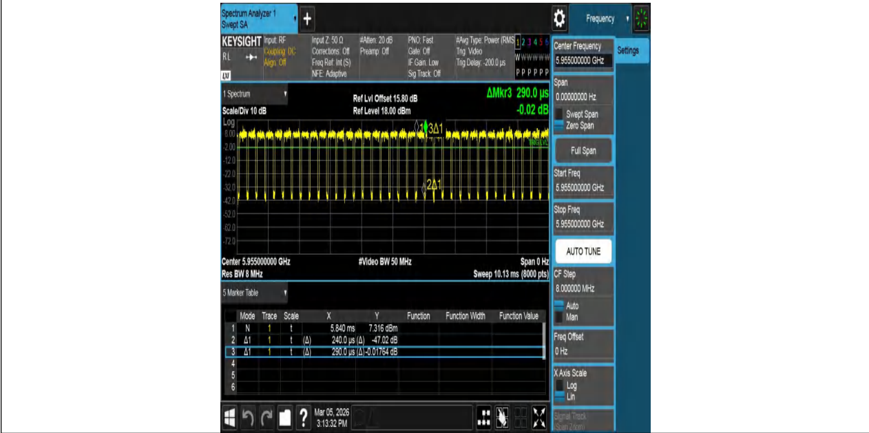
NTNV-11BE20MIMO-Ant2-5955
