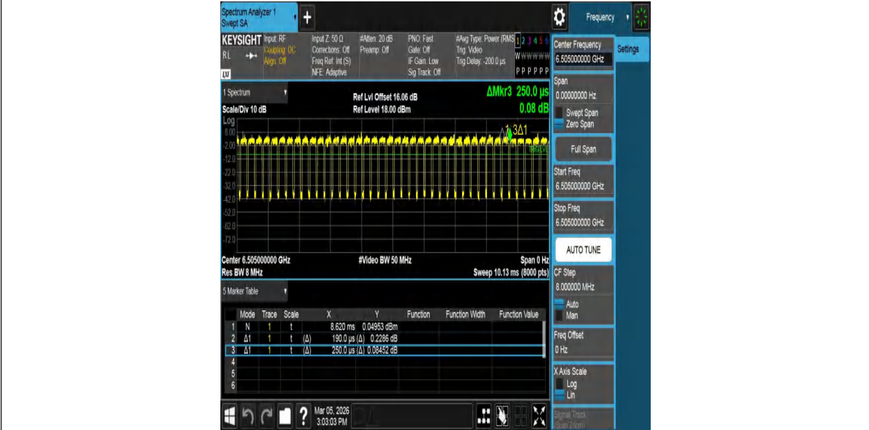
NTNV-11AX160MIMO-Ant2-6505
