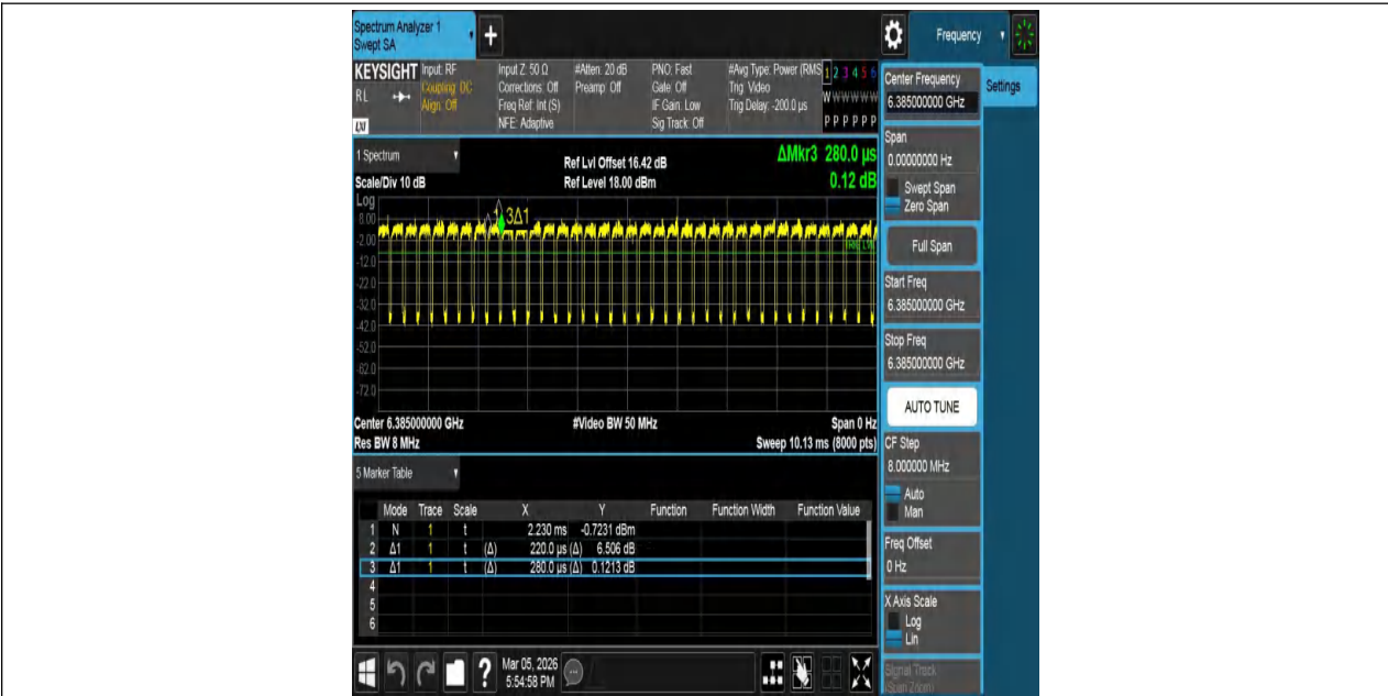
NTNV-11BE80MIMO-Ant1-6385
