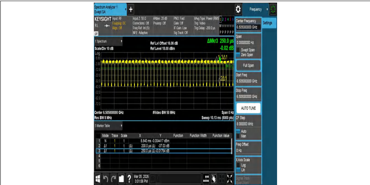
NTNV-11AX160MIMO-Ant1-6505
