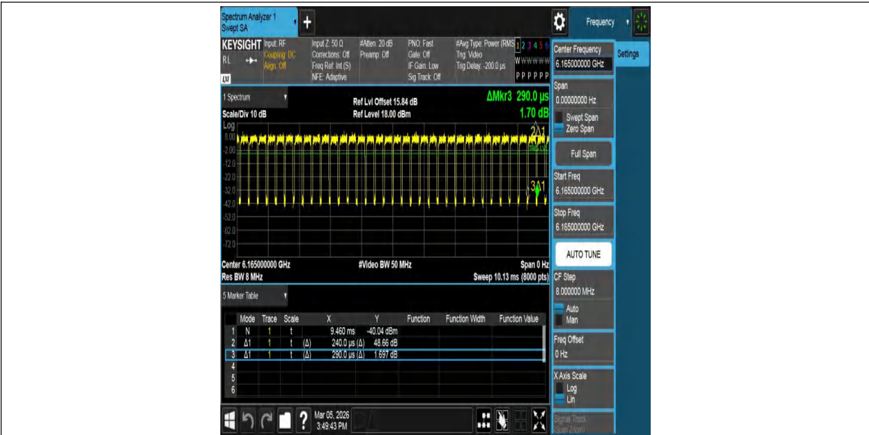
NTNV-11BE40MIMO-Ant1-6165
