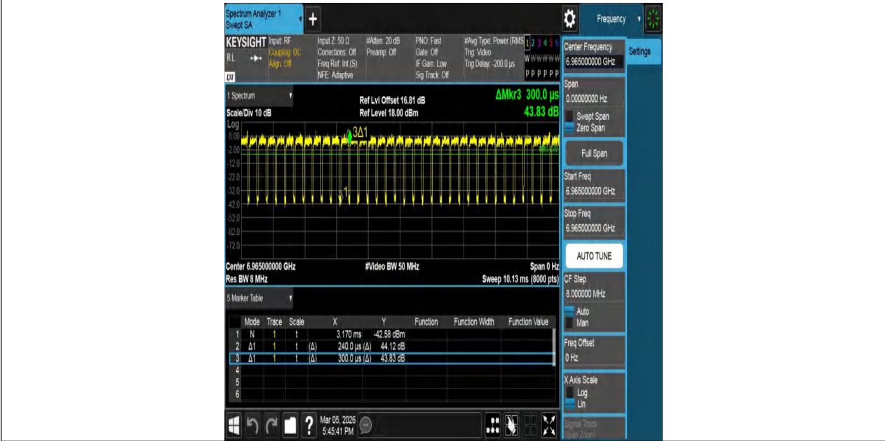
NTNV-11BE40MIMO-Ant2-6965
