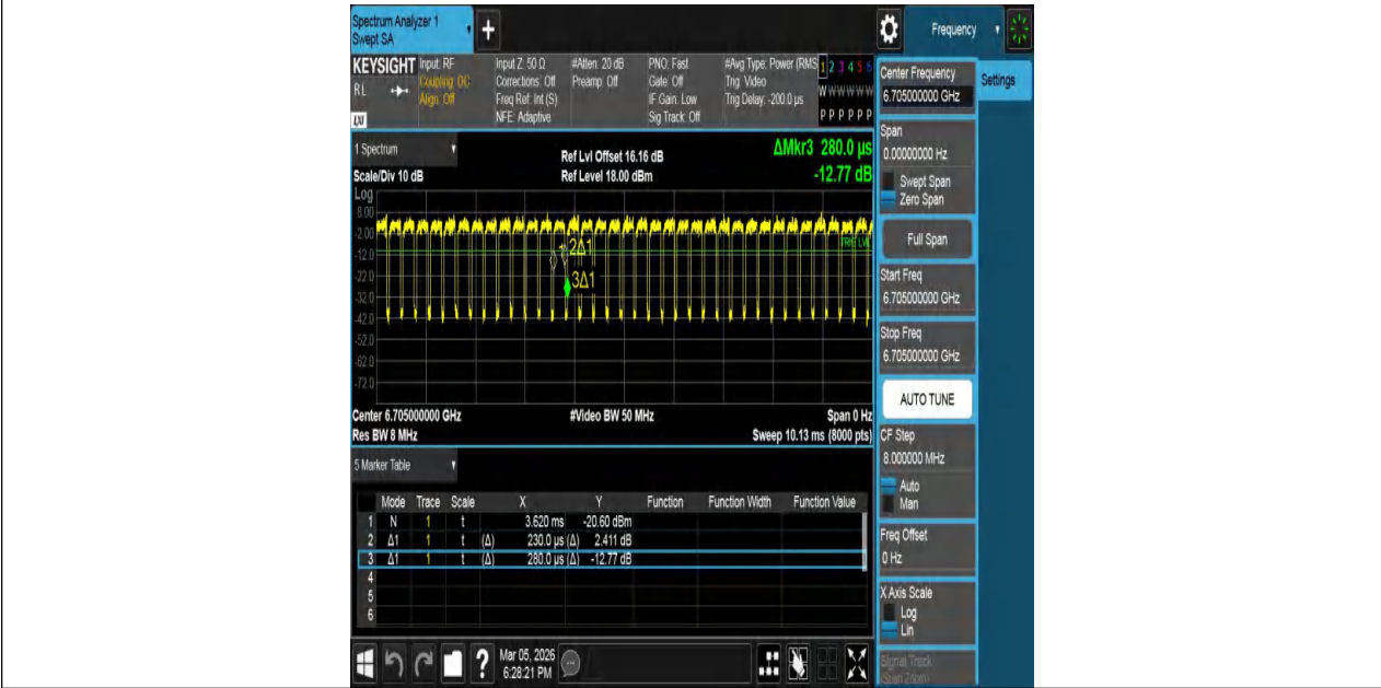
NTNV-11BE80MIMO-Ant2-6705
