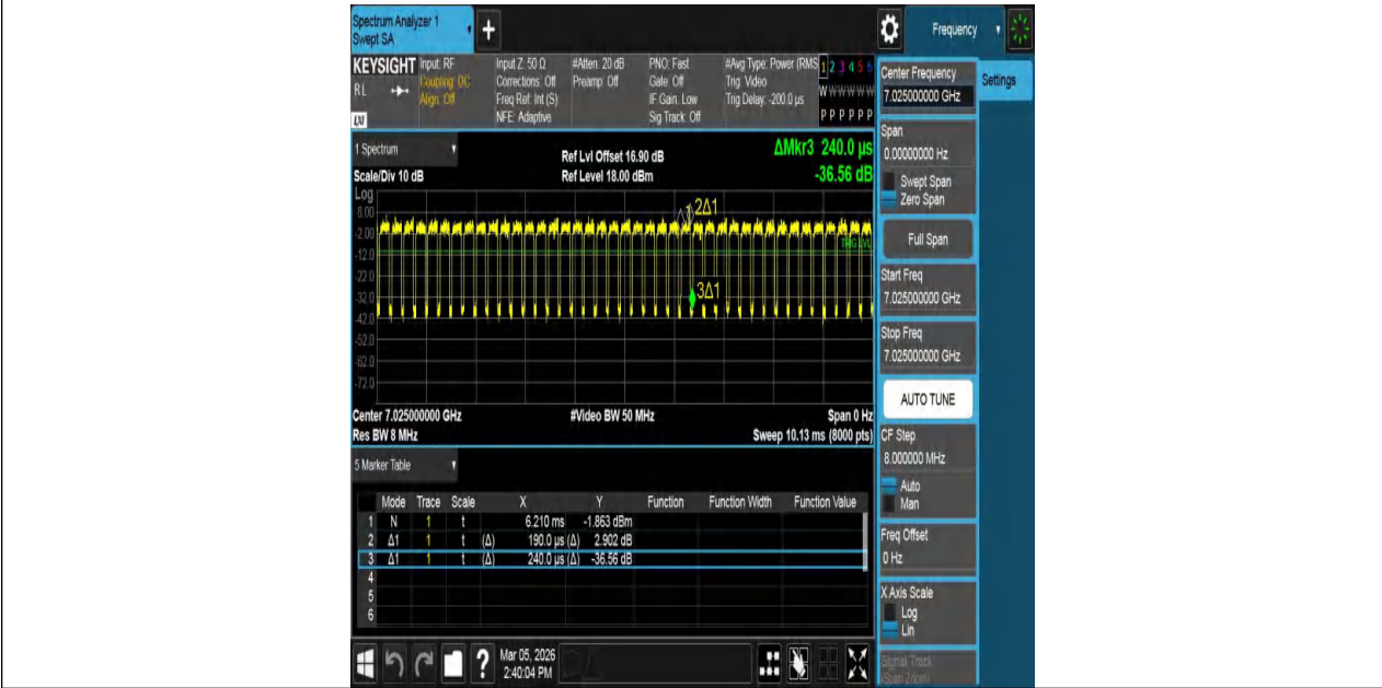
NTNV-11AX80MIMO-Ant2-7025
