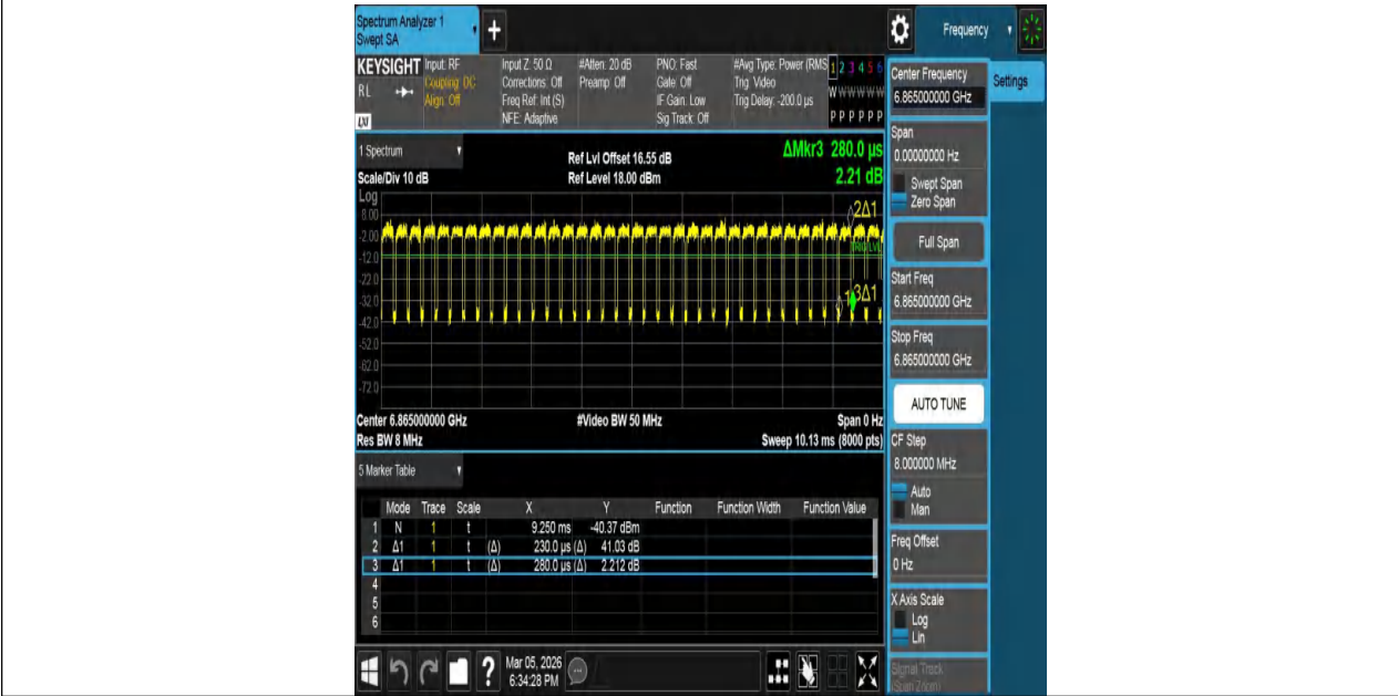
NTNV-11BE80MIMO-Ant2-6865
