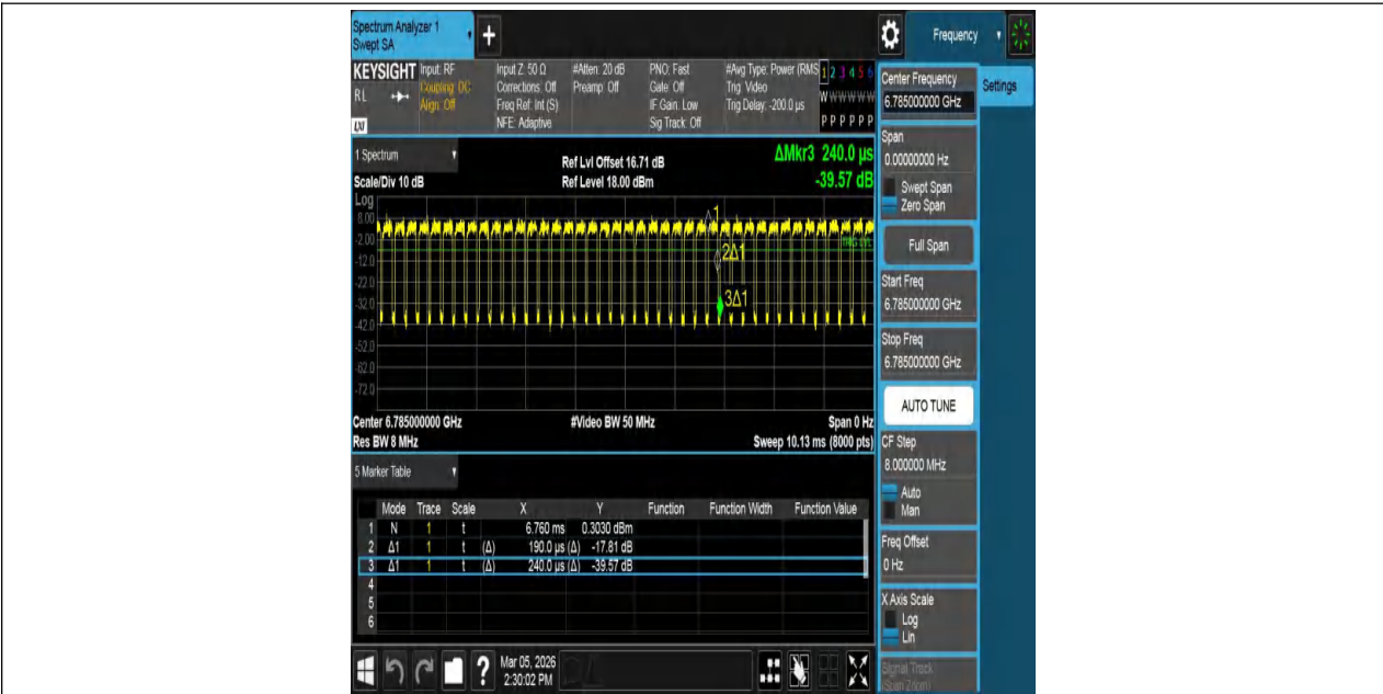
NTNV-11AX80MIMO-Ant1-6785
