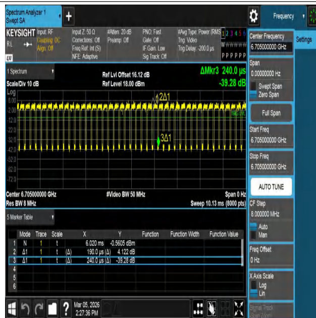
NTNV-11AX80MIMO-Ant1-6705
