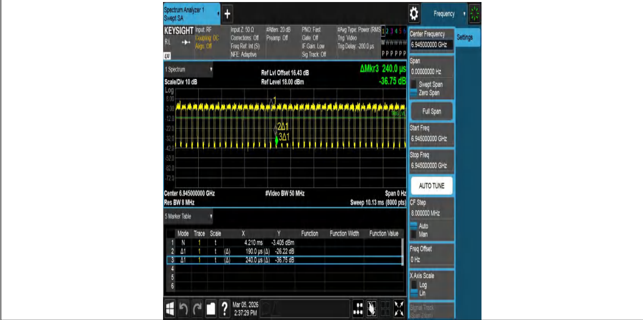
NTNV-11AX80MIMO-Ant2-6945
