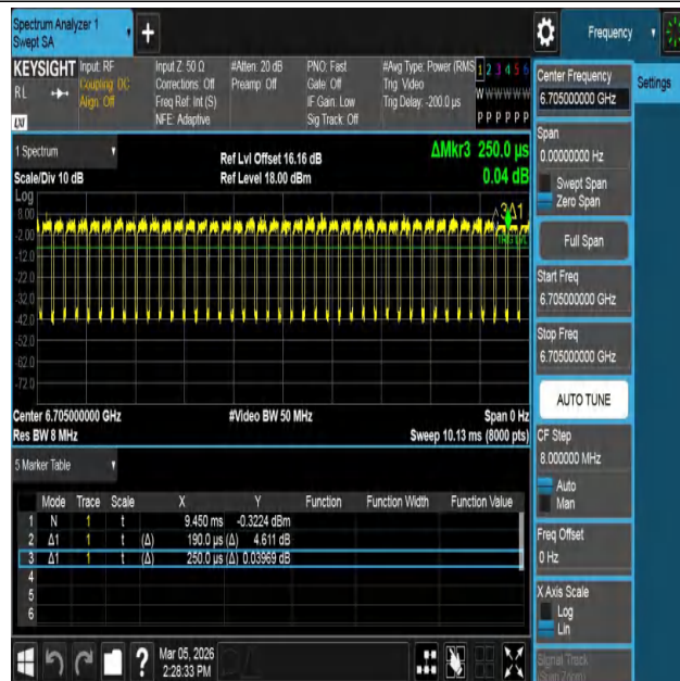
NTNV-11AX80MIMO-Ant2-6705
