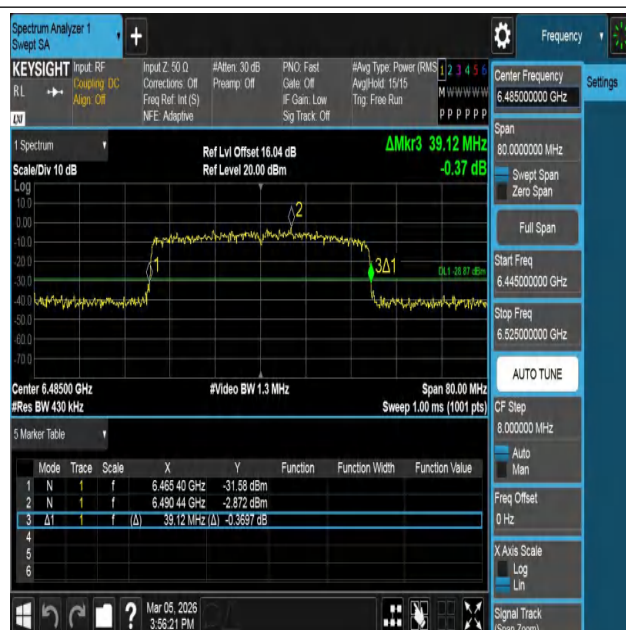
11BE40MIMO-Ant1-6485
