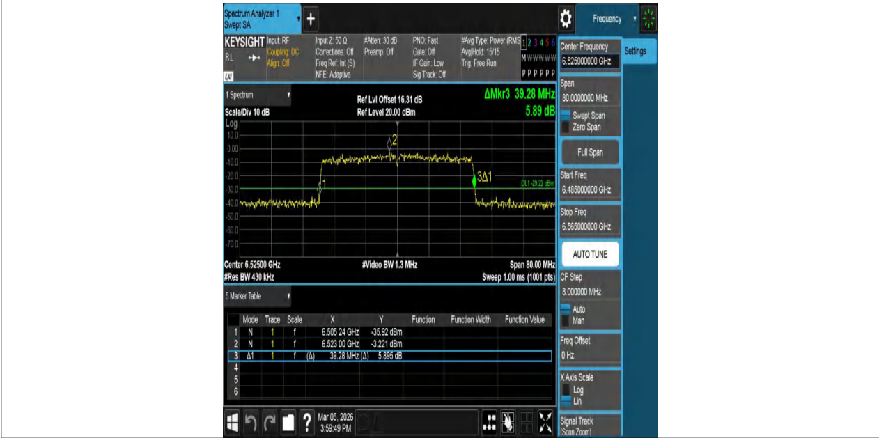
11BE40MIMO-Ant2-6525
