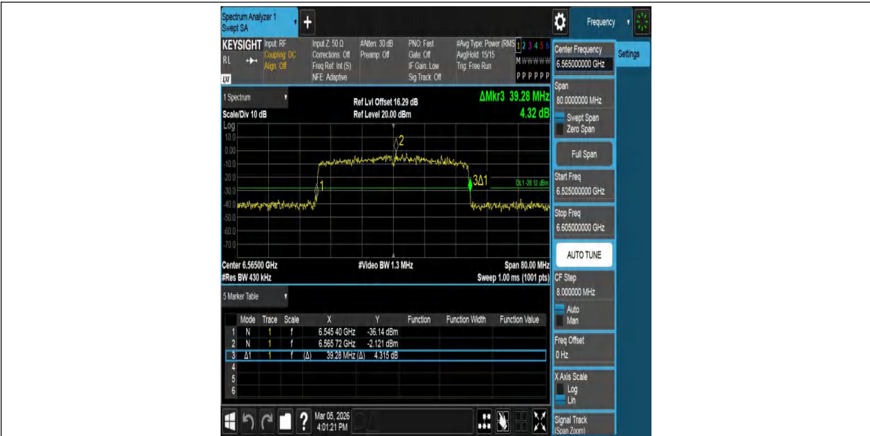
11BE40MIMO-Ant1-6565
