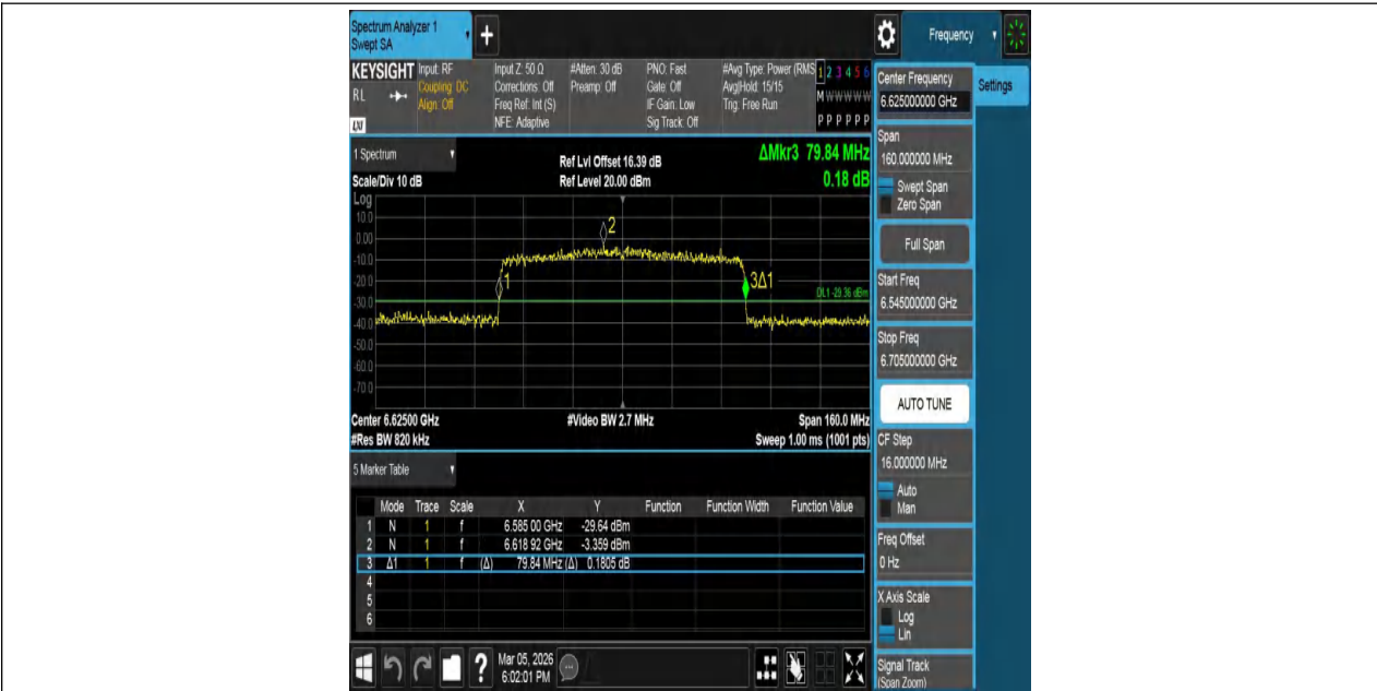
11BE80MIMO-Ant1-6625
