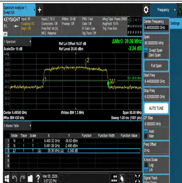
11BE40MIMO-Ant2-6485
