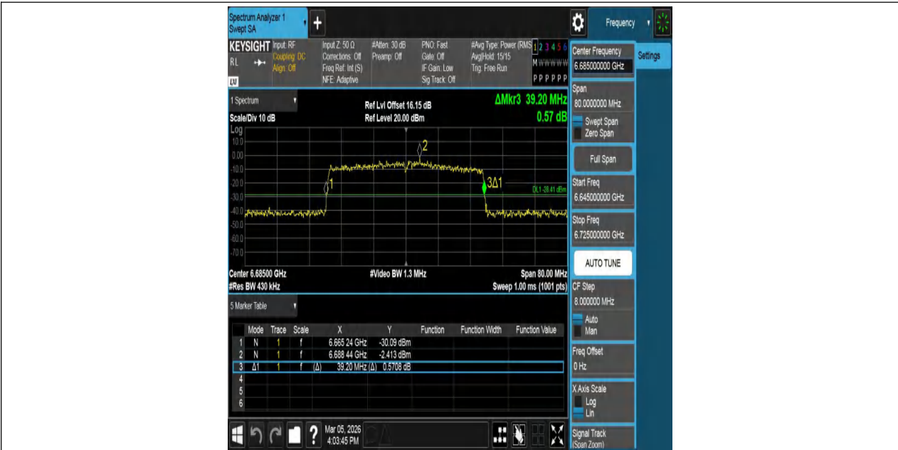
11BE40MIMO-Ant1-6685
