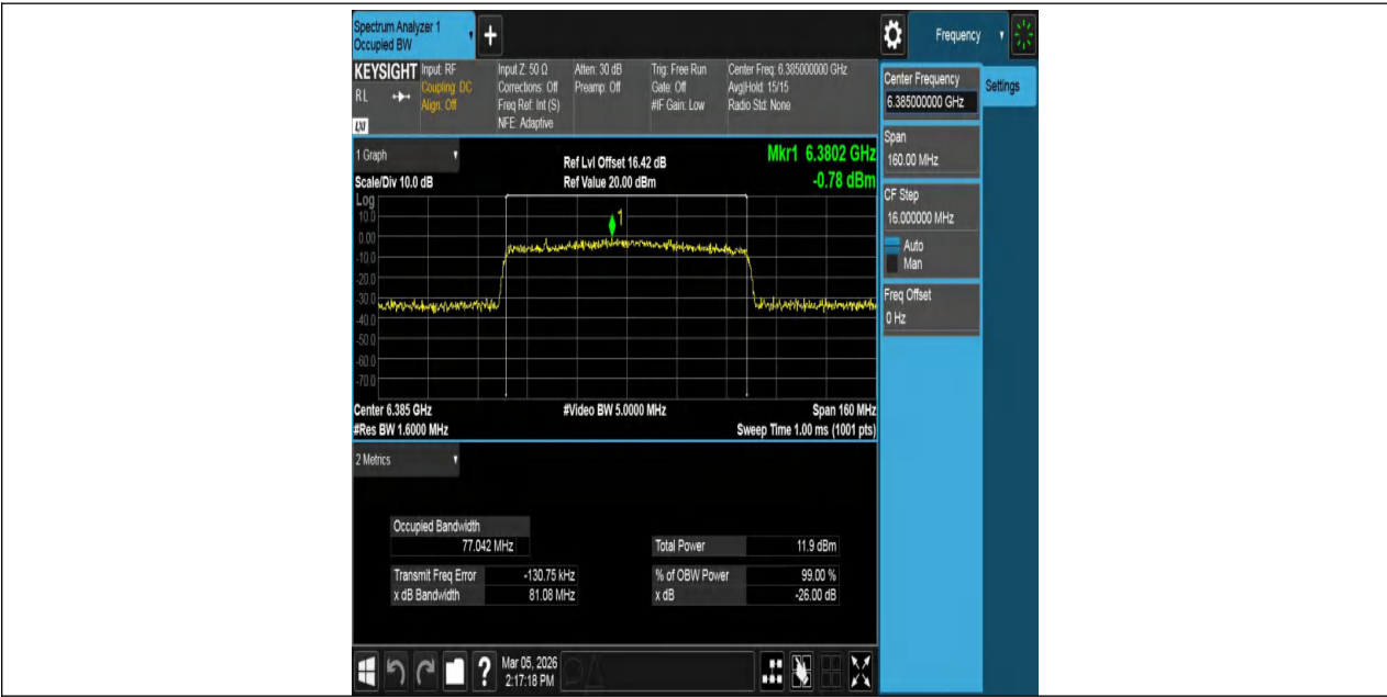
11AX80MIMO-Ant1-6385-PASS
