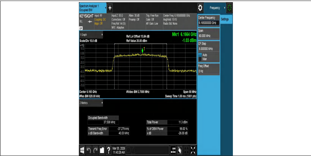
11AX40MIMO-Ant1-6165-PASS
