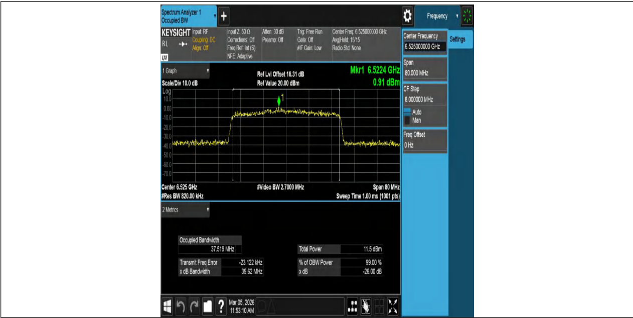
11AX40MIMO-Ant1-6525-PASS
