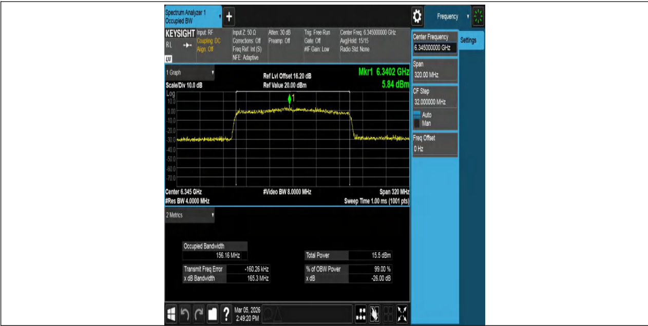
11AX160MIMO-Ant1-6345-PASS
