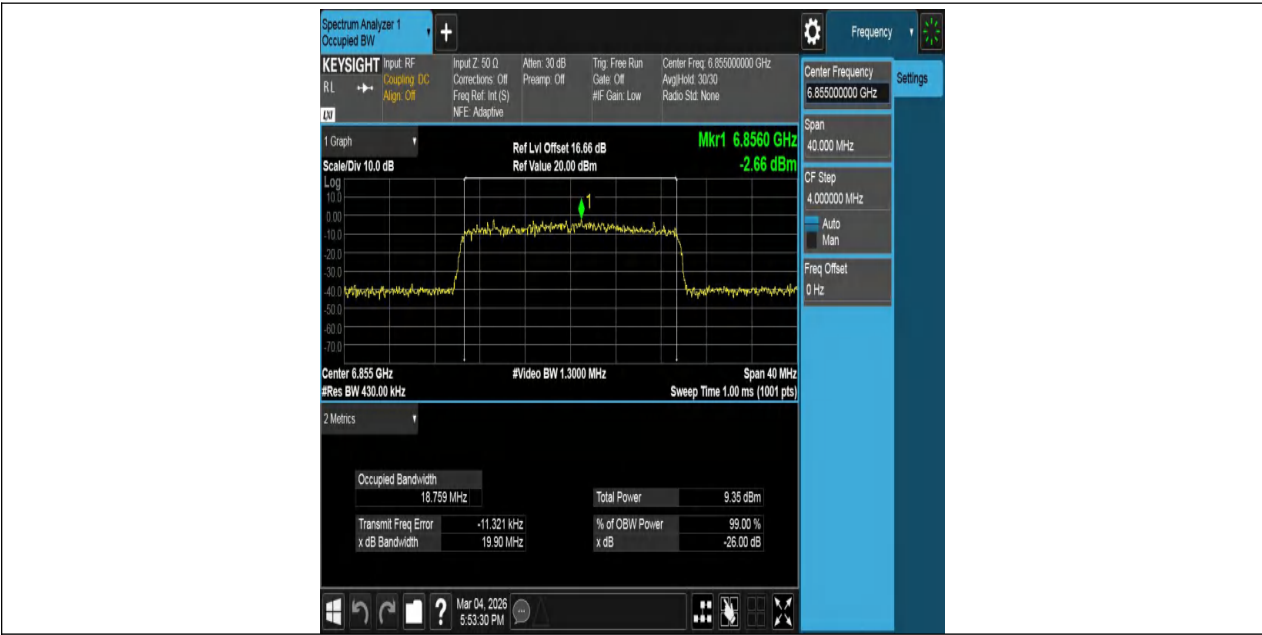
11AX20MIMO-Ant1-6855-PASS
