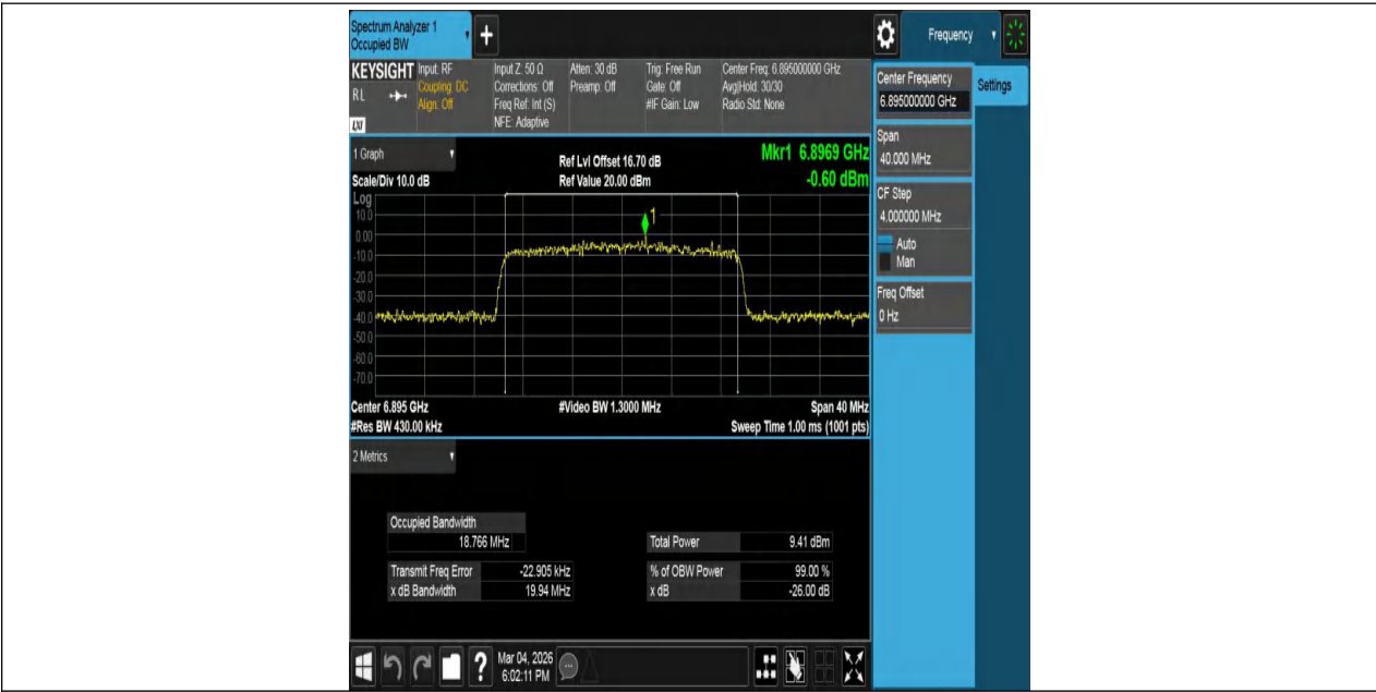
11AX20MIMO-Ant1-6895-PASS
