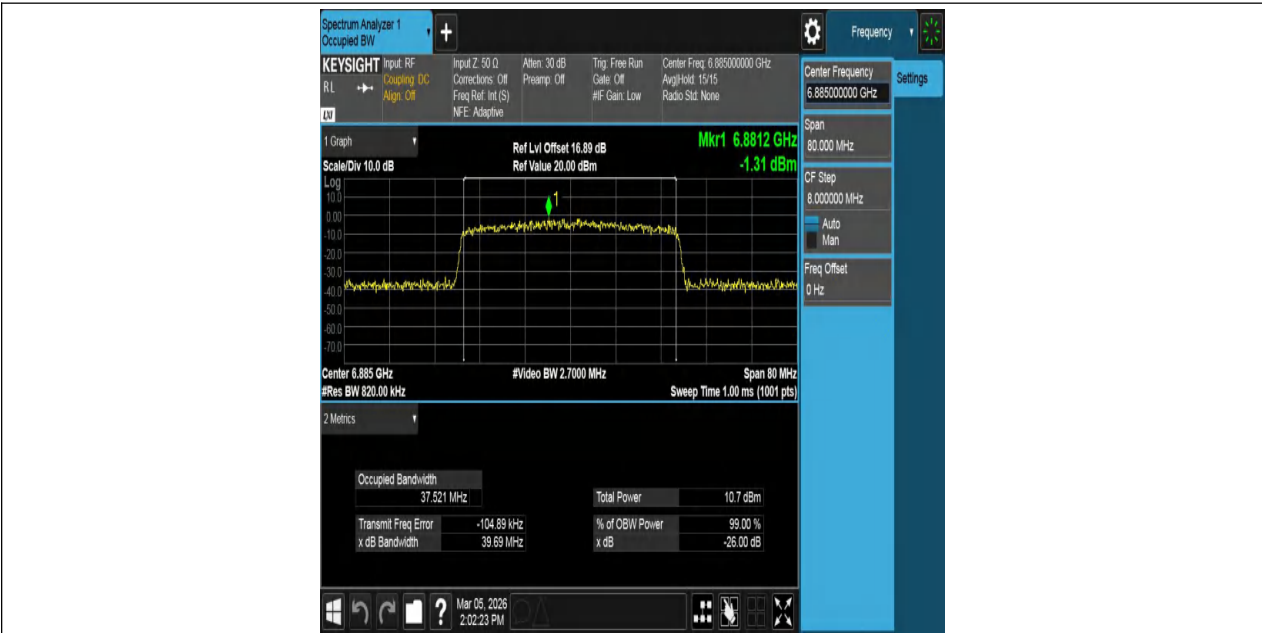
11AX40MIMO-Ant1-6885-PASS
