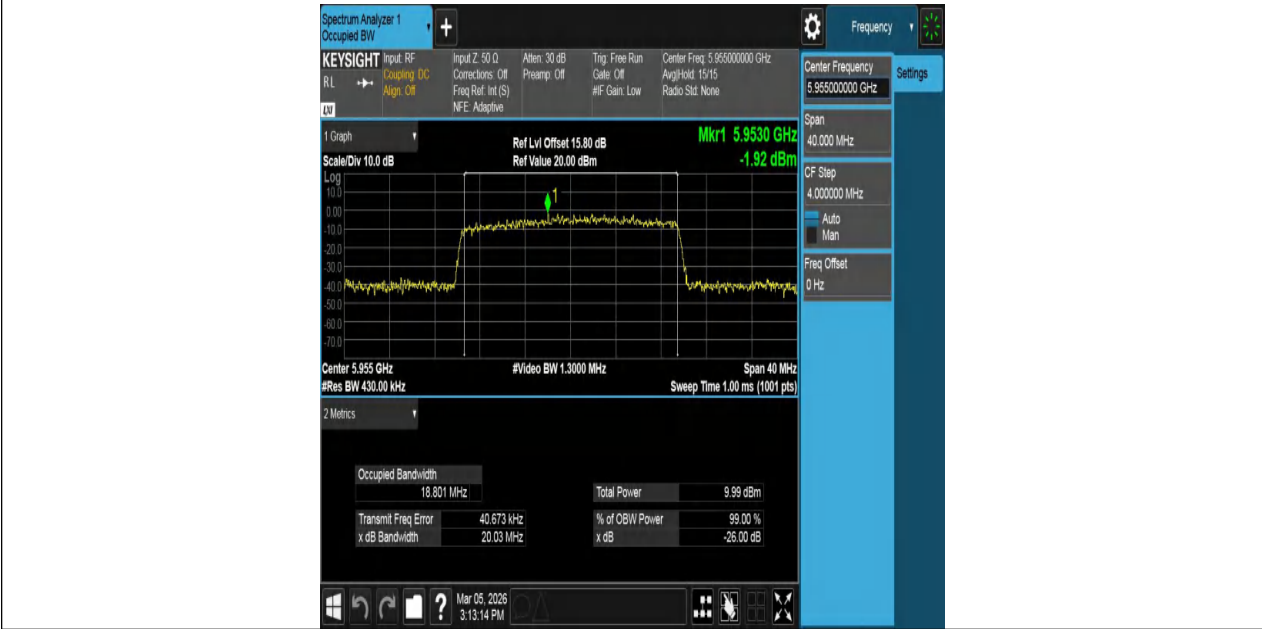
11BE20MIMO-Ant2-5955-PASS
