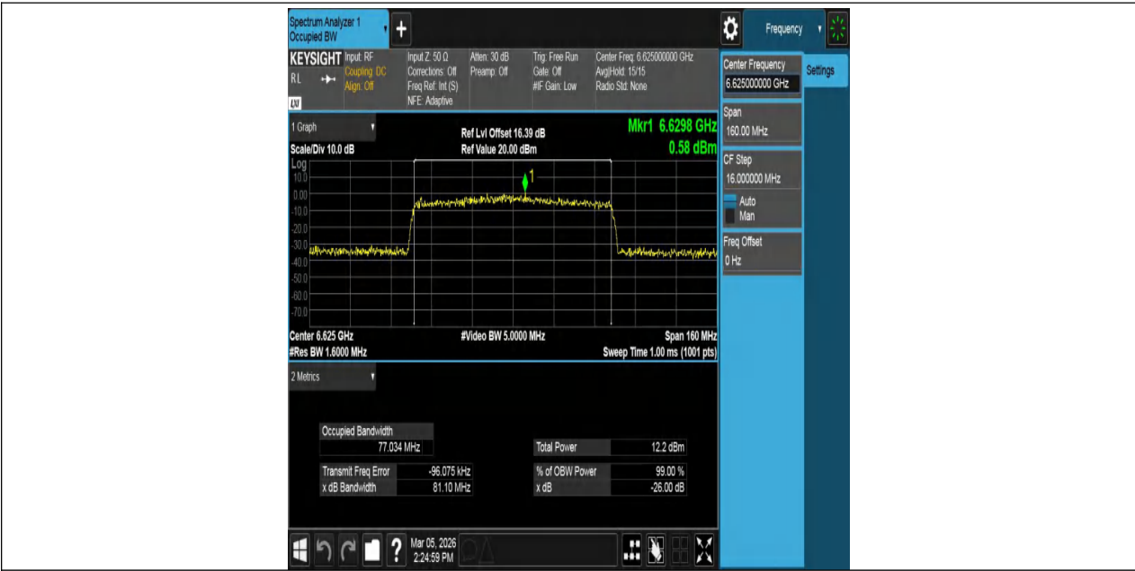
11AX80MIMO-Ant1-6625-PASS
