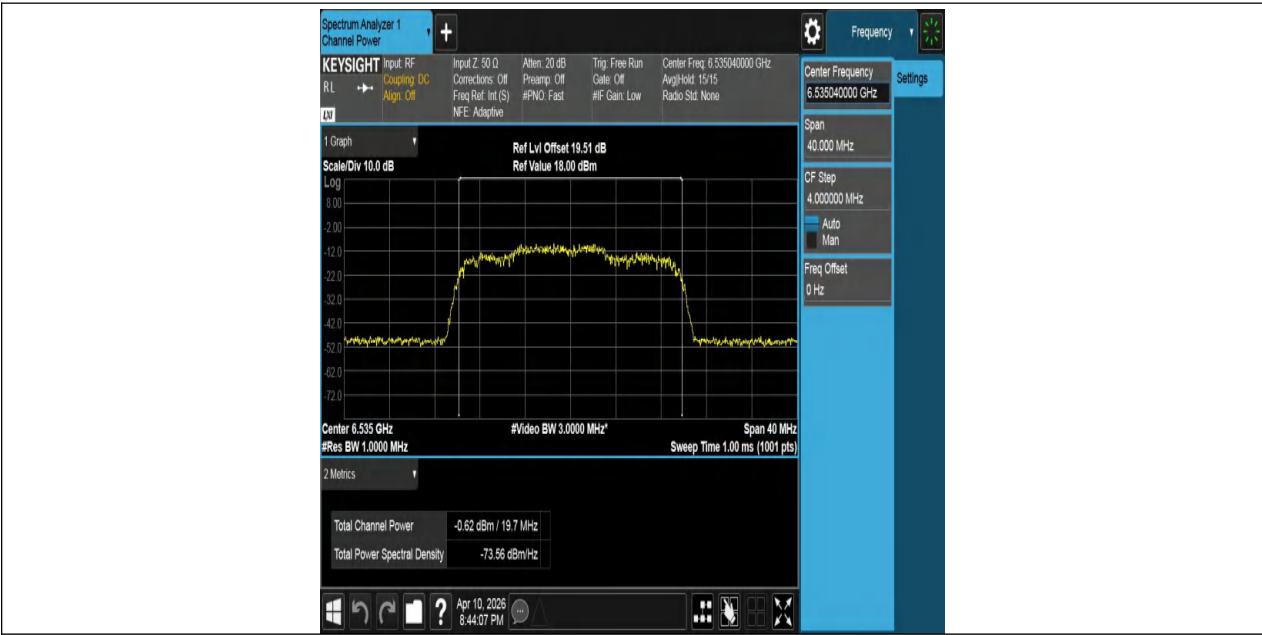
11AX20MIMO-Ant1-6535-PASS
