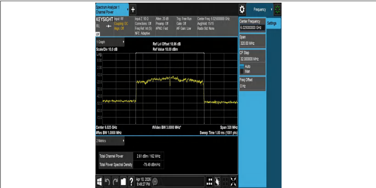
11AX160MIMO-Ant1-6025-PASS
