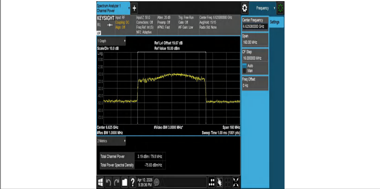
11AX80MIMO-Ant2-6625-PASS
