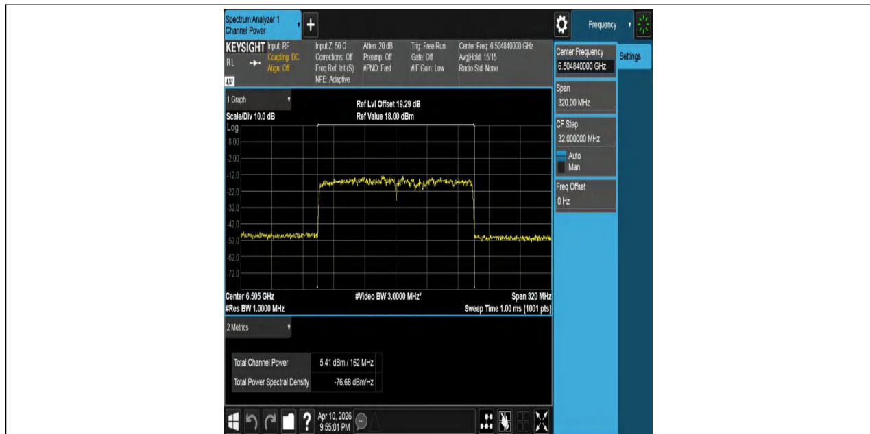
11AX160MIMO-Ant1-6505-PASS
