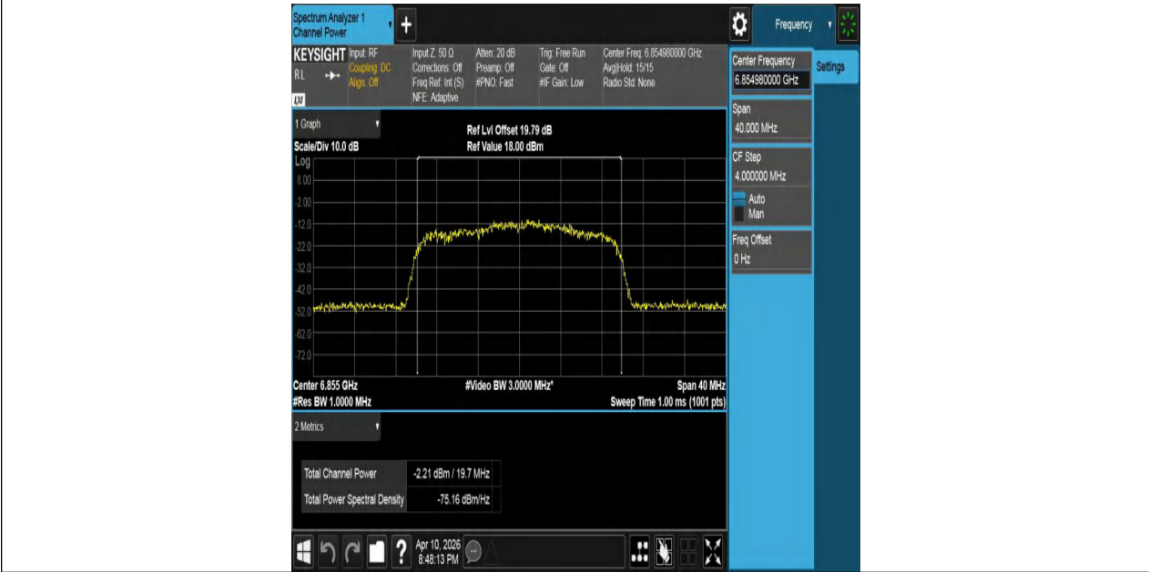
11AX20MIMO-Ant2-6855-PASS
