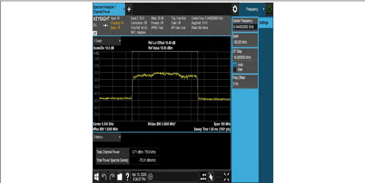
11AX80MIMO-Ant1-6545-PASS
