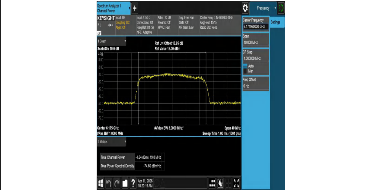
11BE20MIMO-Ant2-6175-PASS
