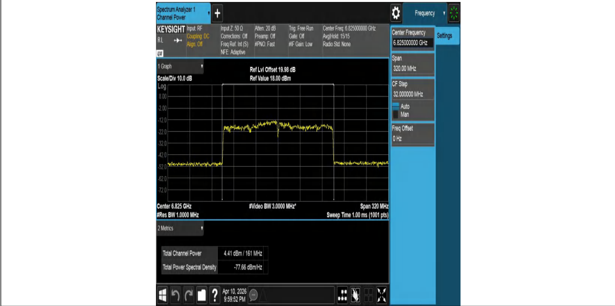
11AX160MIMO-Ant2-6825-PASS
