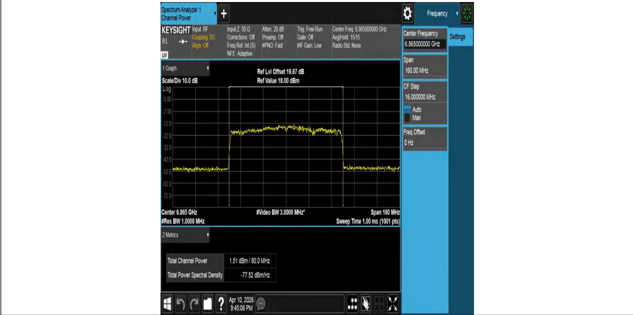
11AX80MIMO-Ant2-6865-PASS
