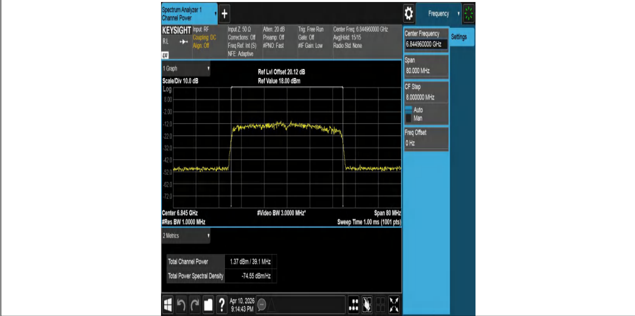
11AX40MIMO-Ant2-6845-PASS
