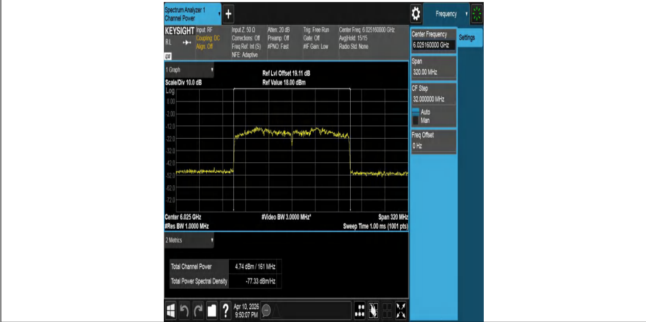
11AX160MIMO-Ant2-6025-PASS
