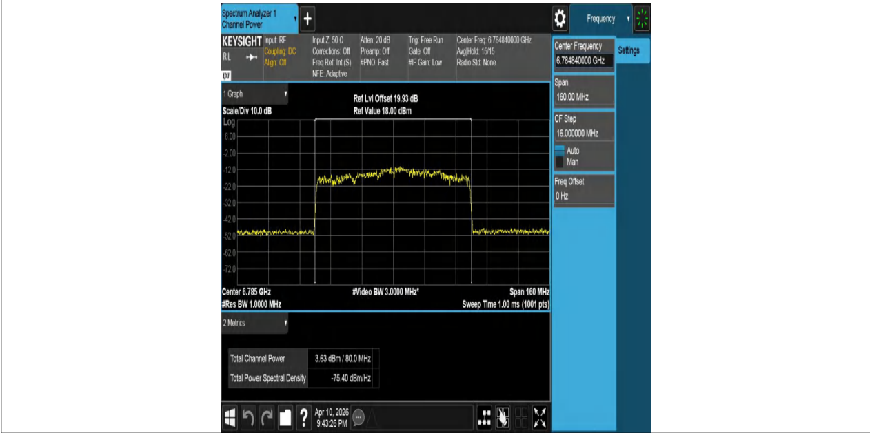
11AX80MIMO-Ant2-6785-PASS
