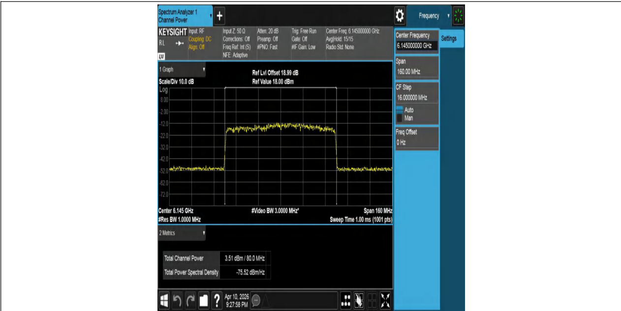
11AX80MIMO-Ant1-6145-PASS
