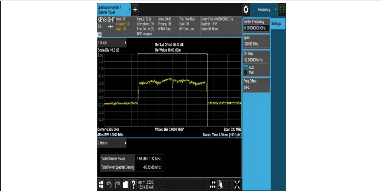
11AX160MIMO-Ant1-6985-PASS
