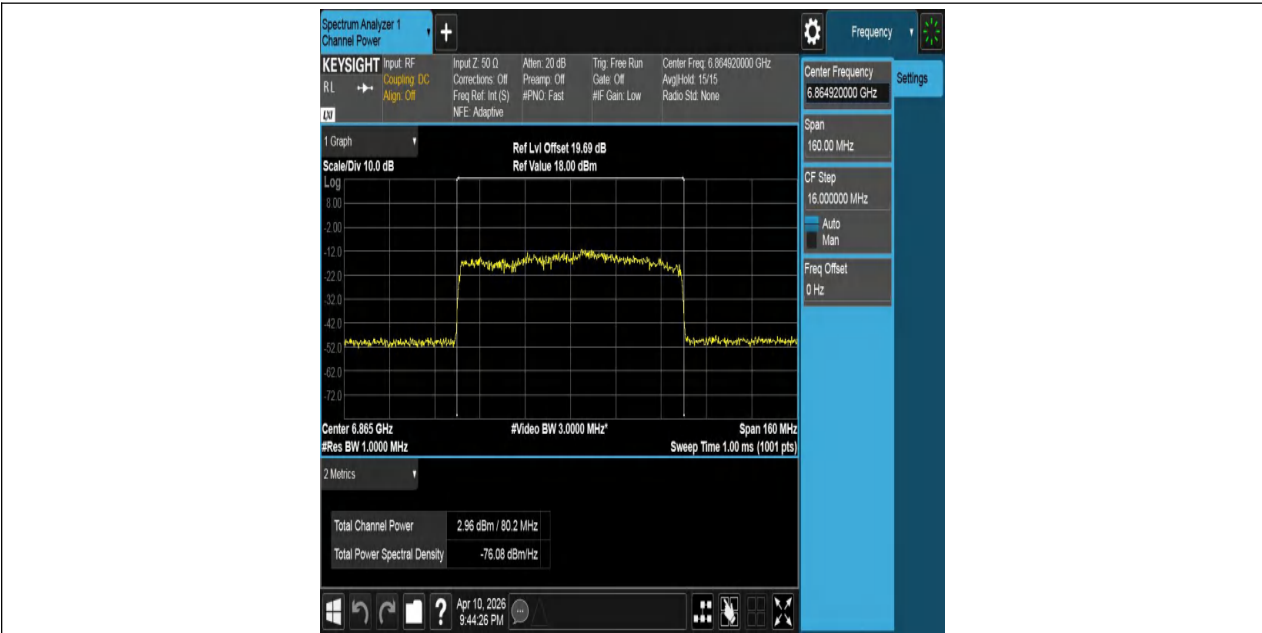
11AX80MIMO-Ant1-6865-PASS
