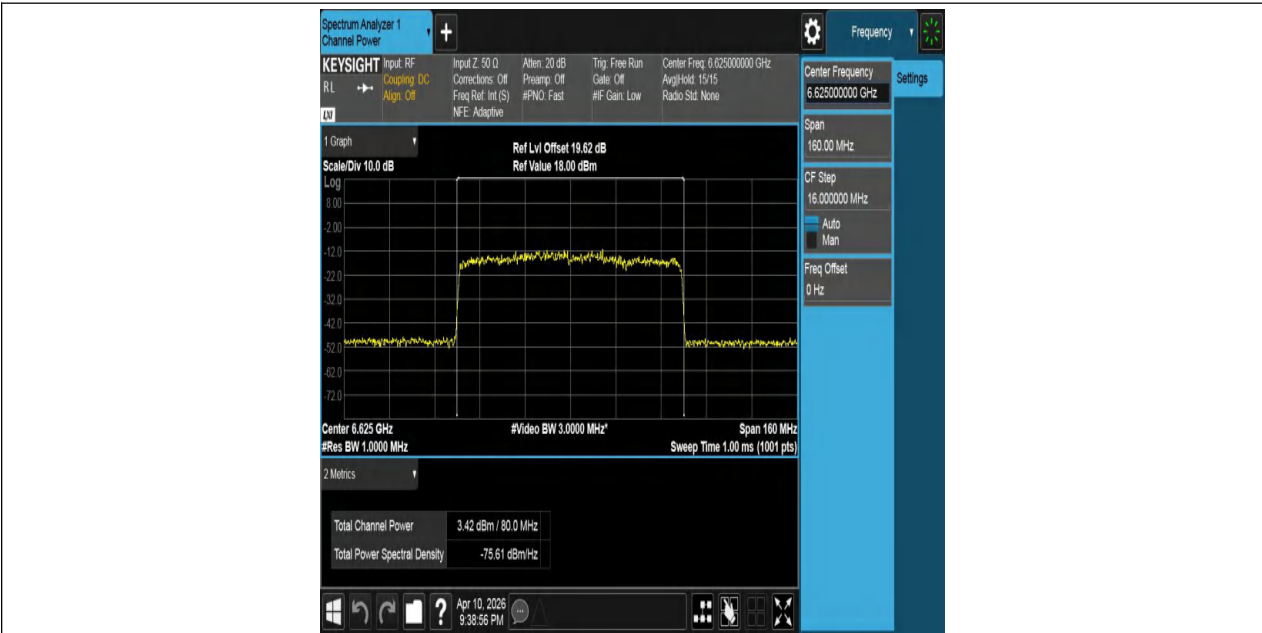
11AX80MIMO-Ant1-6625-PASS
