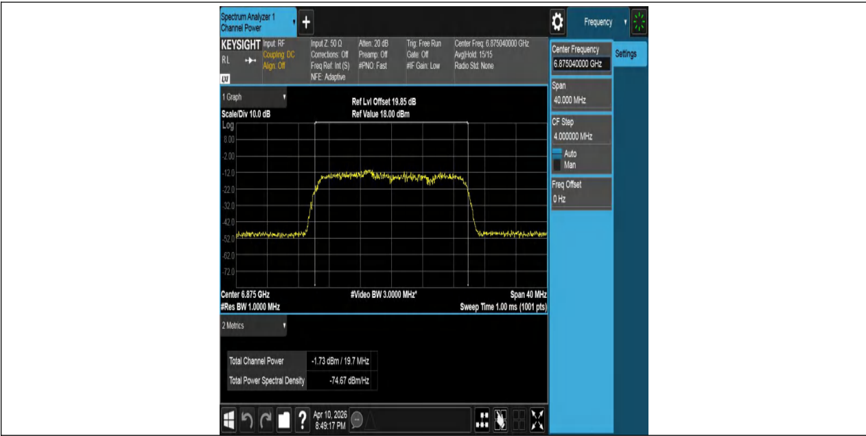
11AX20MIMO-Ant1-6875-PASS
