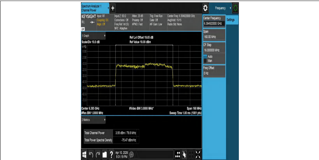
11AX80MIMO-Ant1-6385-PASS
