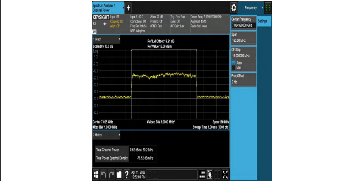
11AX80MIMO-Ant2-7025-PASS
