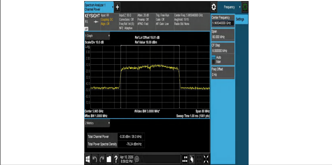
11AX40MIMO-Ant1-5965-PASS
