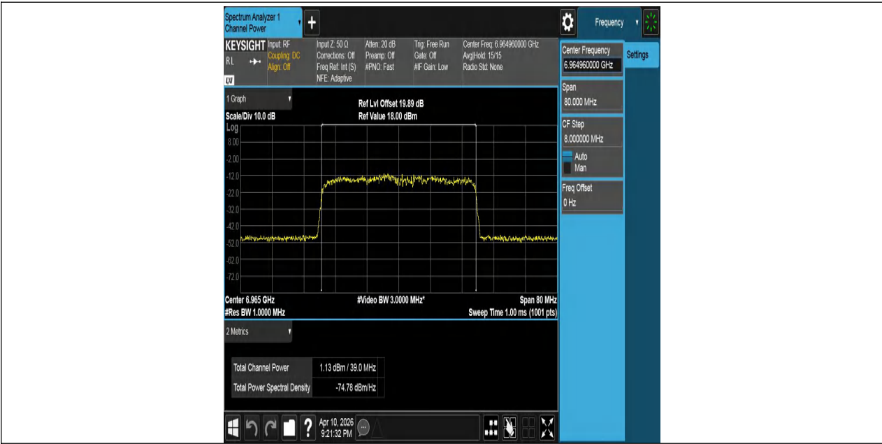
11AX40MIMO-Ant1-6965-PASS
