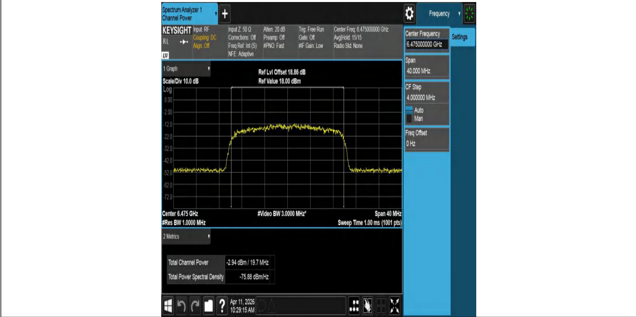
11BE20MIMO-Ant2-6475-PASS
