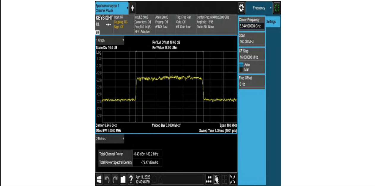
11AX80MIMO-Ant2-6945-PASS
