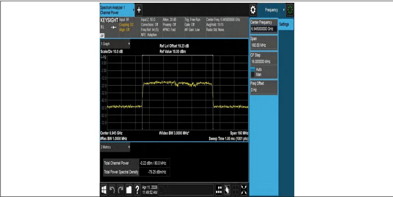
11BE80MIMO-Ant1-6945-PASS
