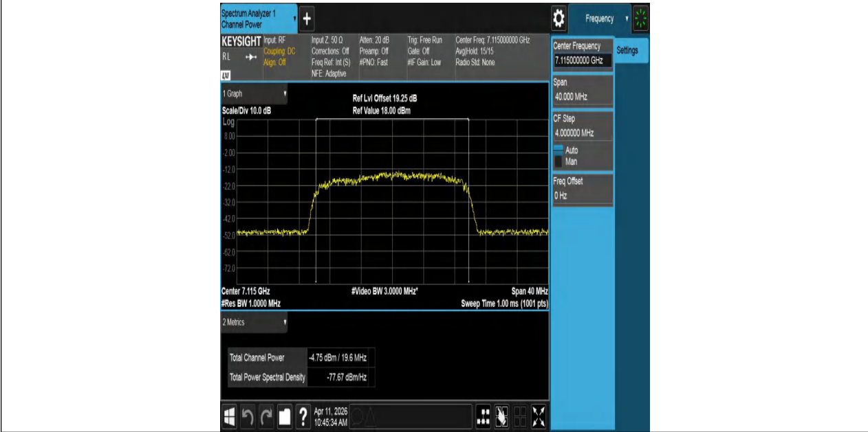
11BE20MIMO-Ant2-7115-PASS
