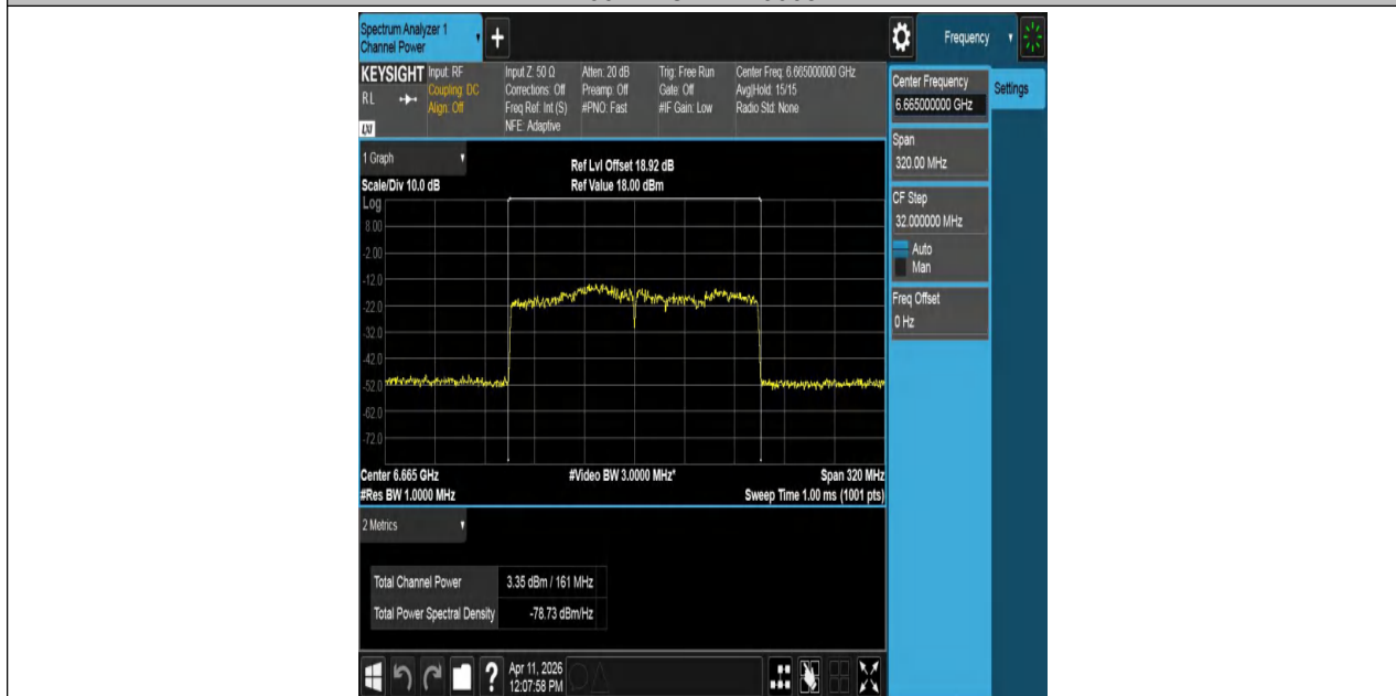
11BE160MIMO-Ant2-6665-PASS
