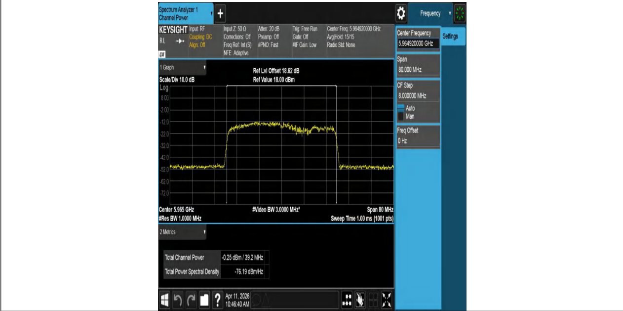
11BE40MIMO-Ant1-5965-PASS
