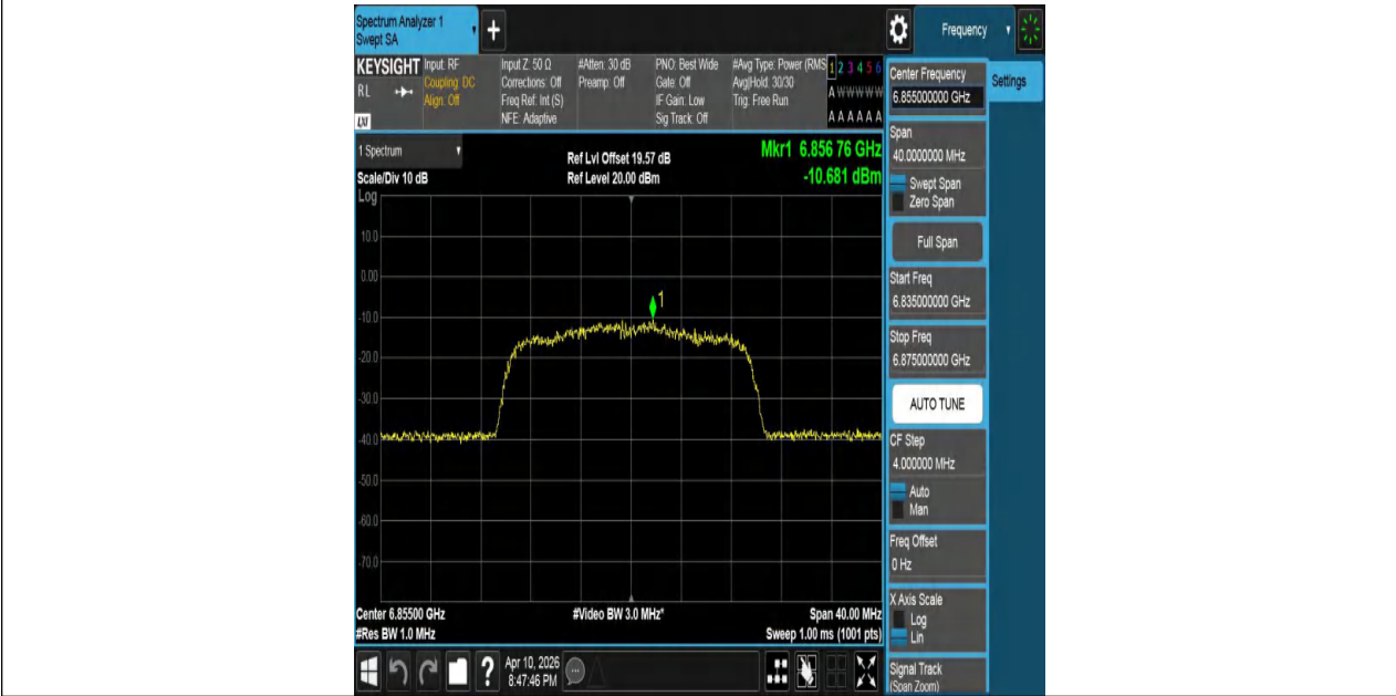
11AX20MIMO-Ant1-6855-PASS
