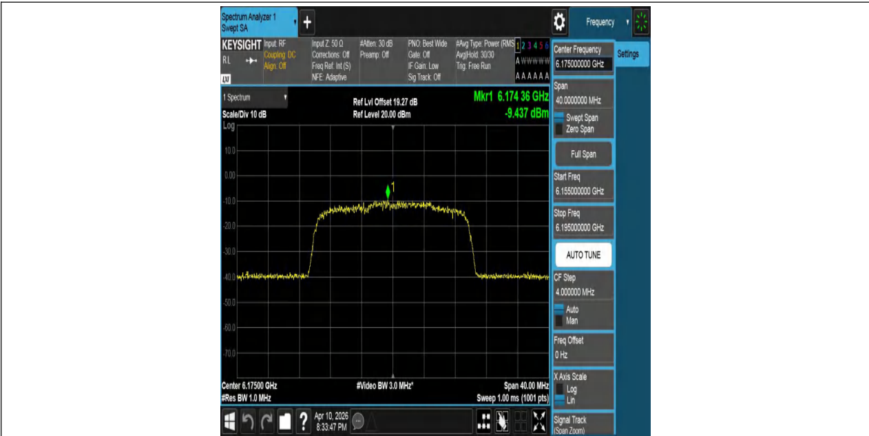
11AX20MIMO-Ant1-6175-PASS
