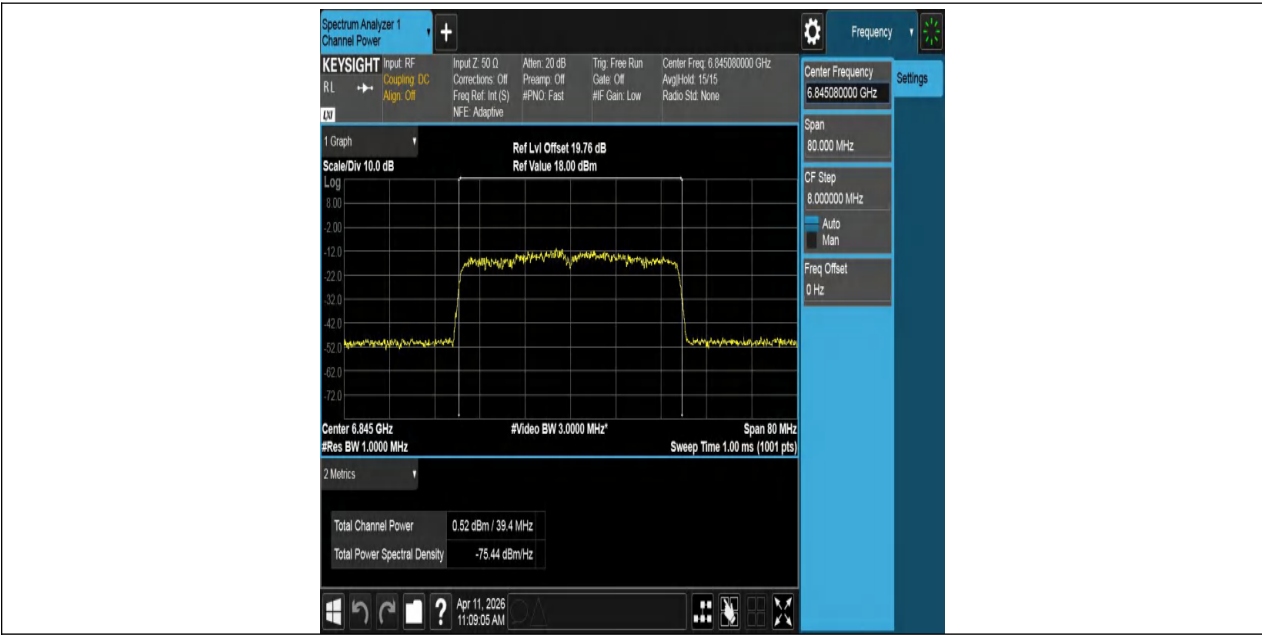
11BE40MIMO-Ant1-6845-PASS
