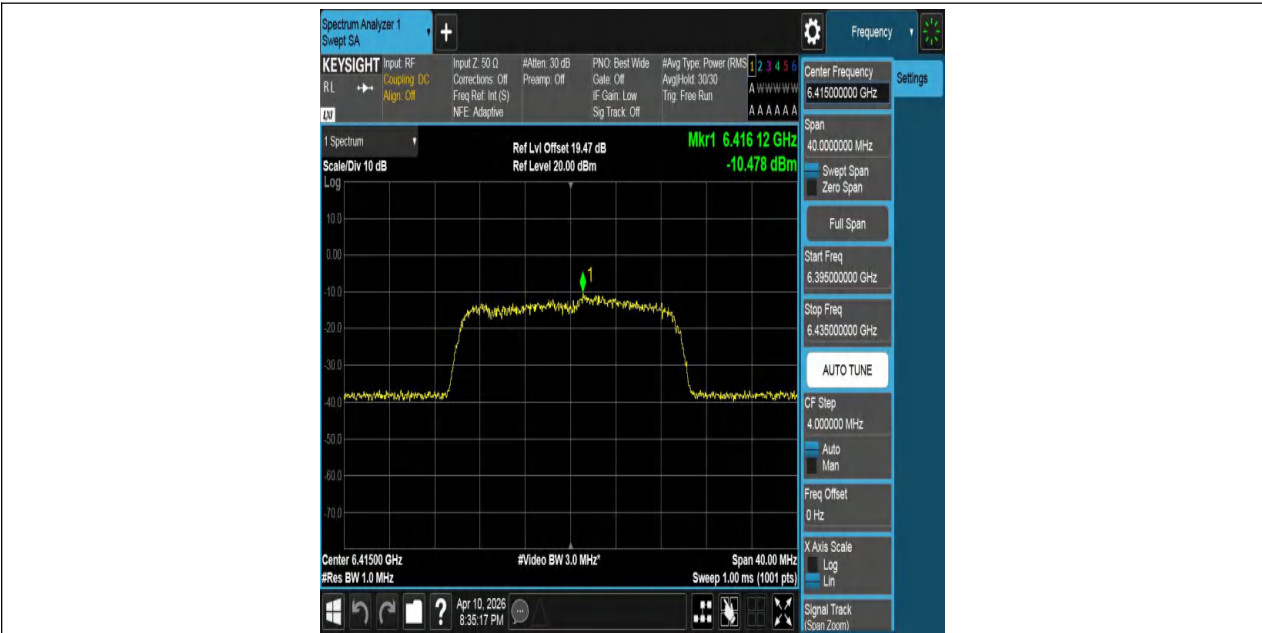
11AX20MIMO-Ant1-6415-PASS
