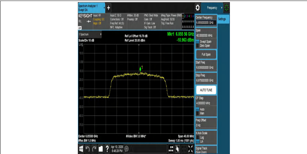
11AX20MIMO-Ant2-6855-PASS
