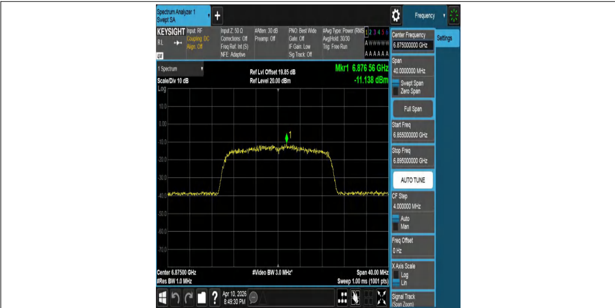
11AX20MIMO-Ant1-6875-PASS
