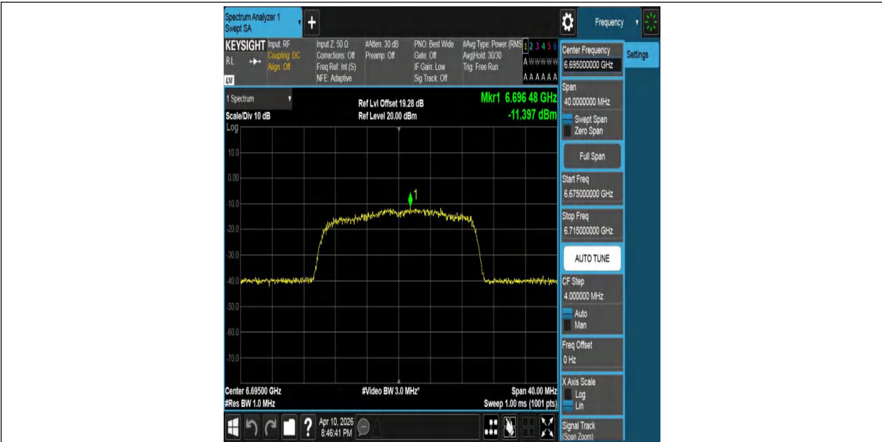
11AX20MIMO-Ant2-6695-PASS
