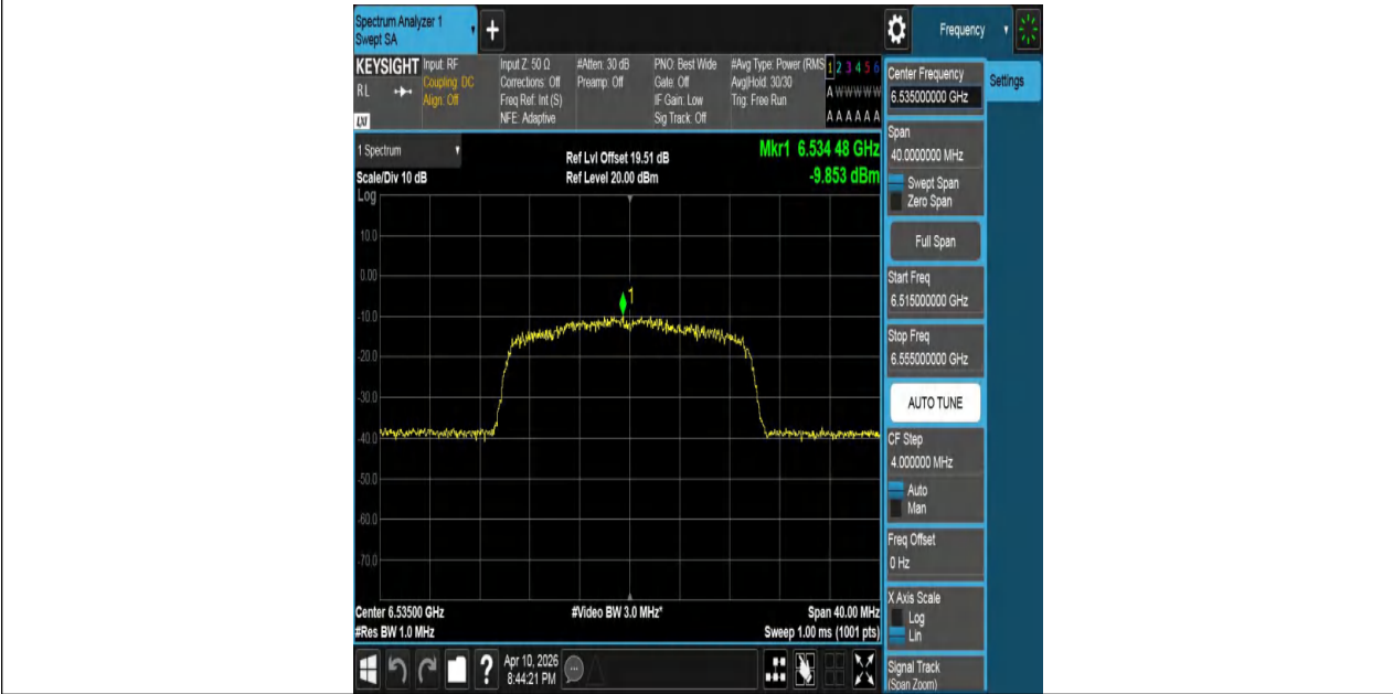
11AX20MIMO-Ant1-6535-PASS
