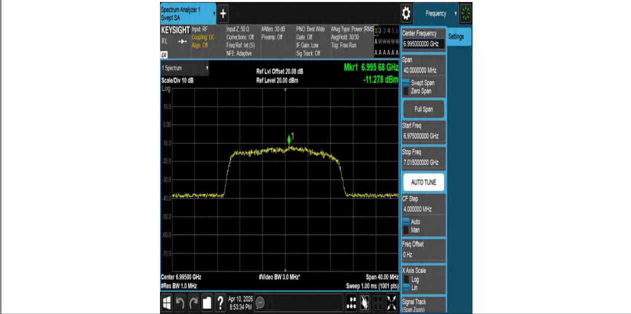
11AX20MIMO-Ant2-6995-PASS
