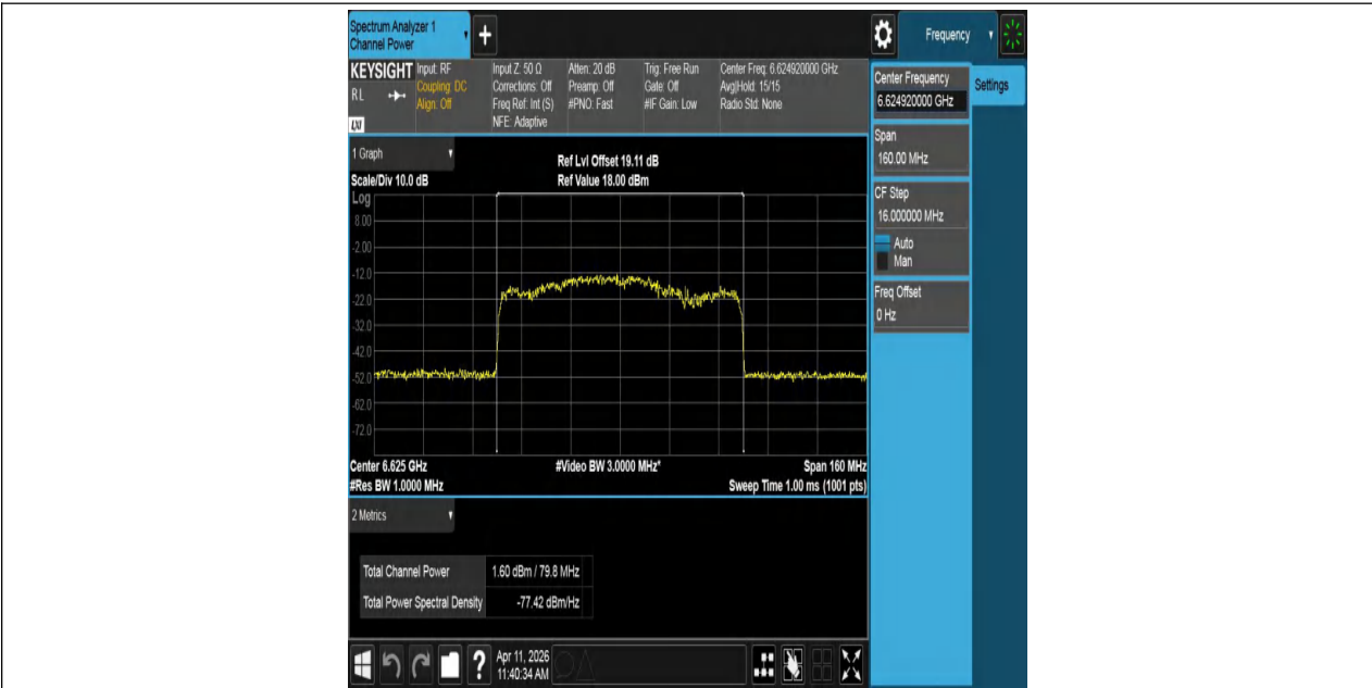
11BE80MIMO-Ant1-6625-PASS
