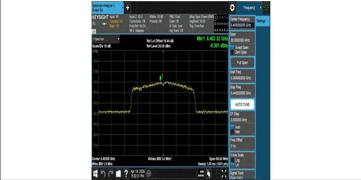
11AX40MIMO-Ant1-6405-PASS
