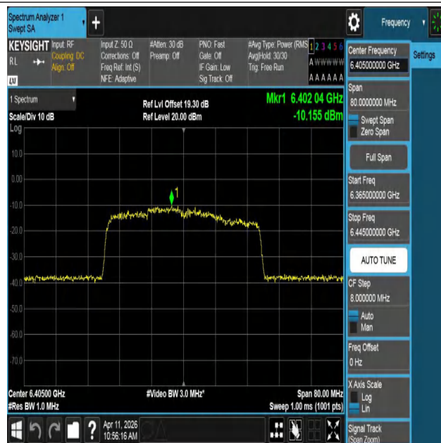
11BE40MIMO-Ant2-6405-PASS
