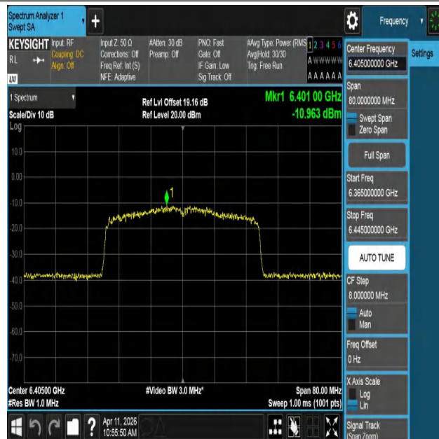
11BE40MIMO-Ant1-6405-PASS
