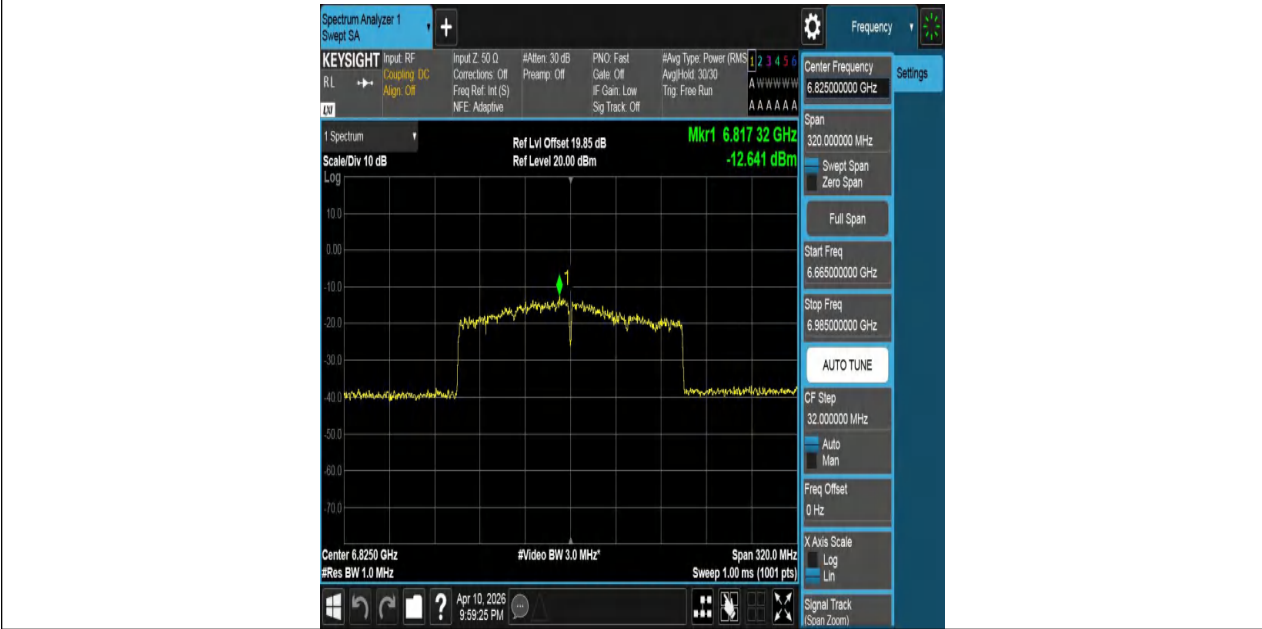
11AX160MIMO-Ant1-6825-PASS
