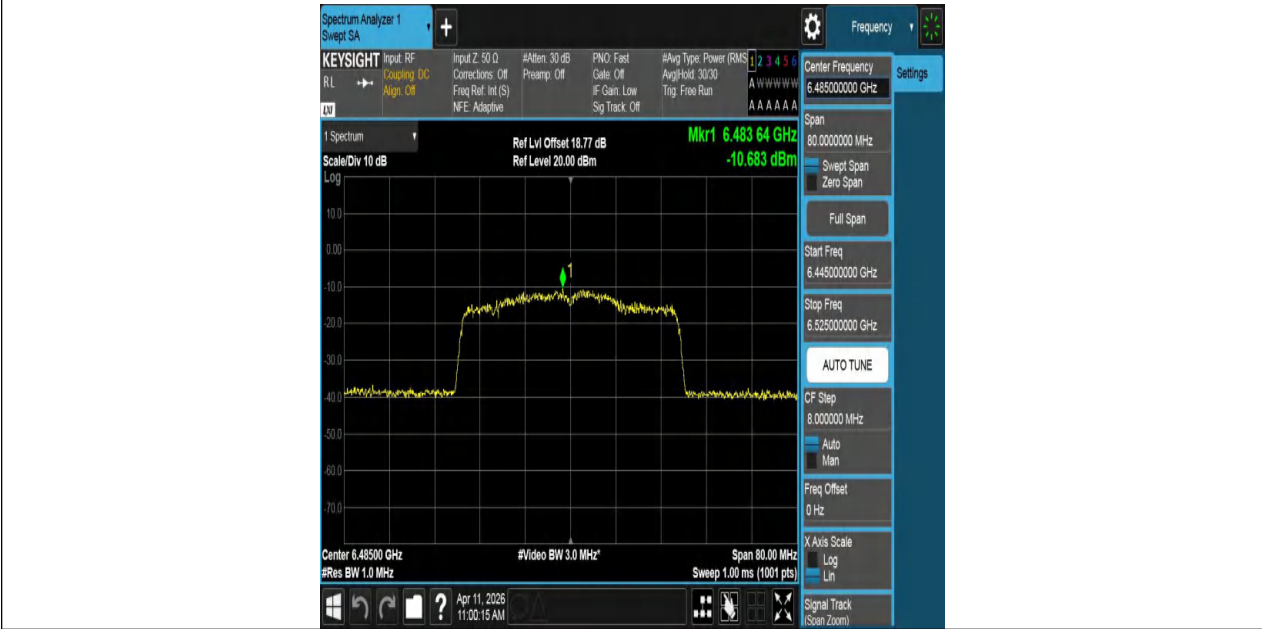
11BE40MIMO-Ant1-6485-PASS
