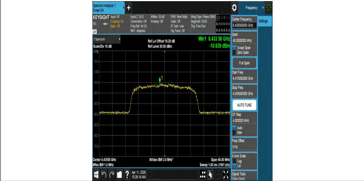
11BE20MIMO-Ant2-6435-PASS
