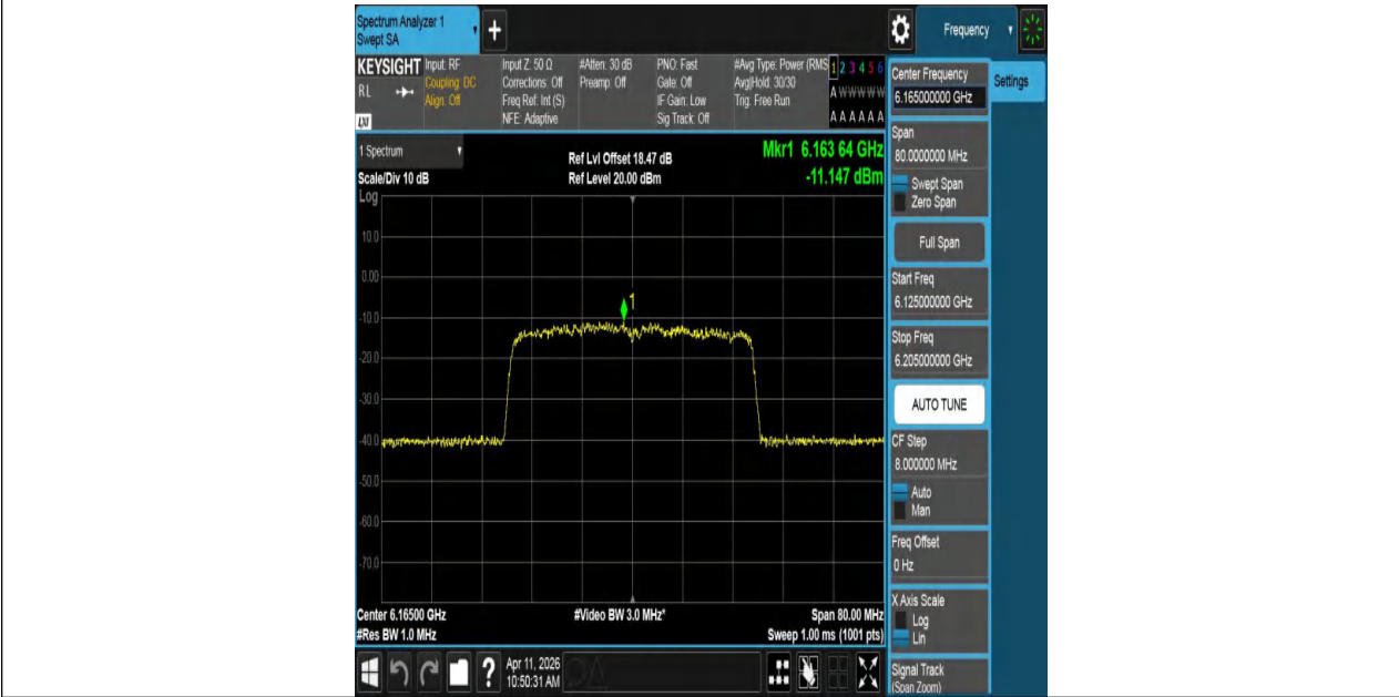
11BE40MIMO-Ant1-6165-PASS
