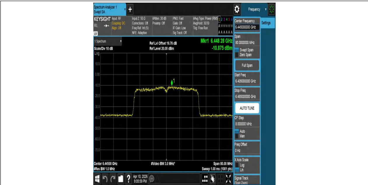
11AX40MIMO-Ant2-6445-PASS
