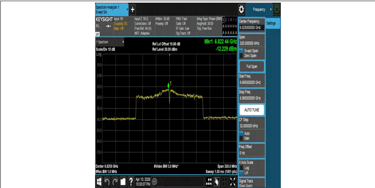
11AX160MIMO-Ant2-6825-PASS
