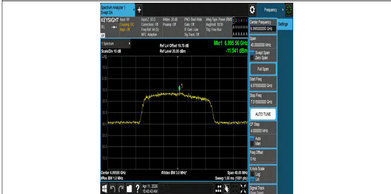
11BE20MIMO-Ant2-6995-PASS
