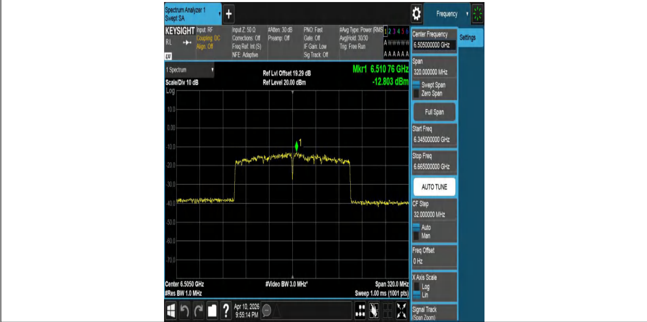
11AX160MIMO-Ant1-6505-PASS
