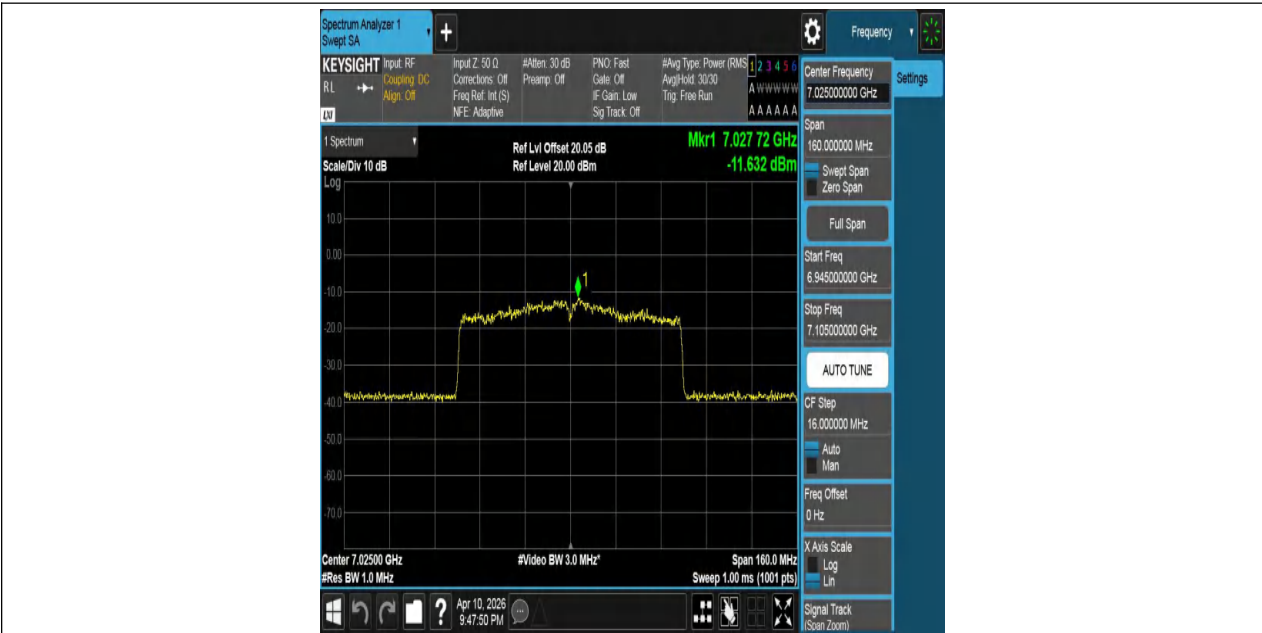
11AX80MIMO-Ant1-7025-PASS
