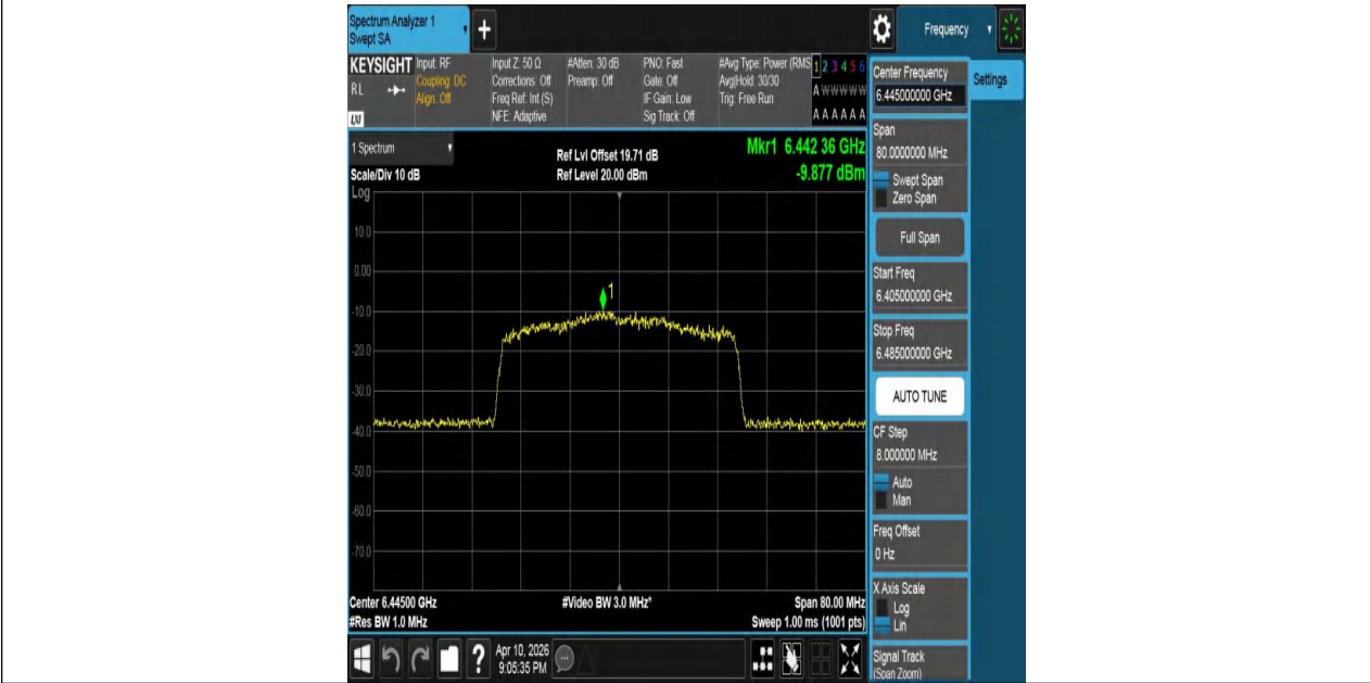
11AX40MIMO-Ant1-6445-PASS
