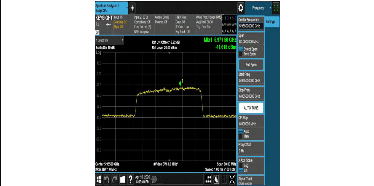
11AX40MIMO-Ant2-5965-PASS
