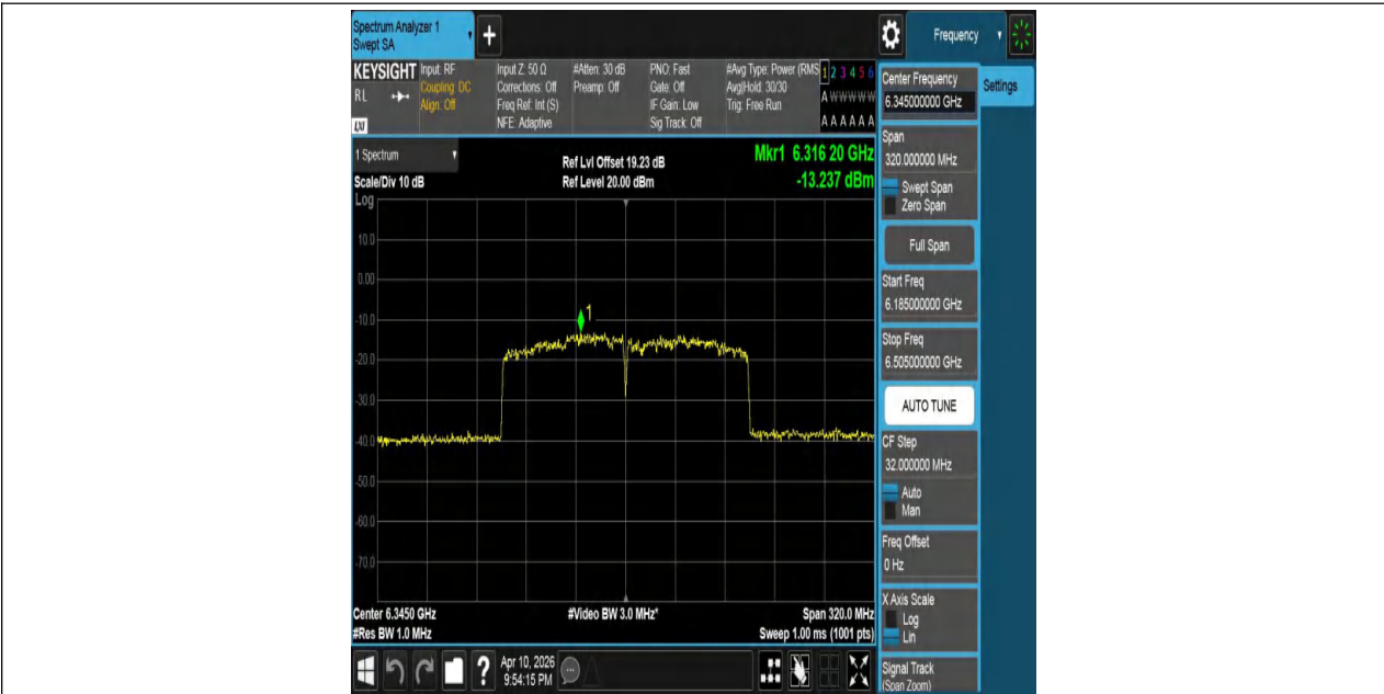
11AX160MIMO-Ant2-6345-PASS
