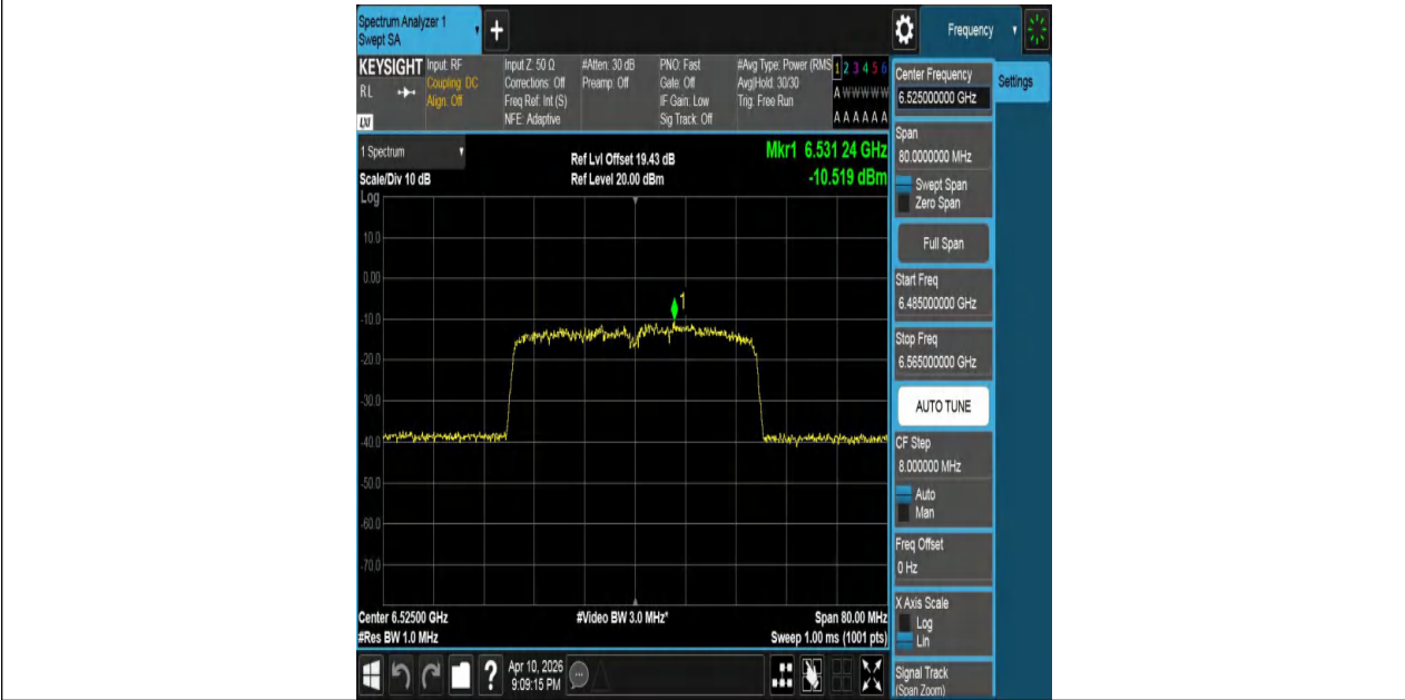
11AX40MIMO-Ant1-6525-PASS
