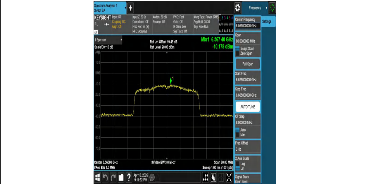
11AX40MIMO-Ant2-6565-PASS
