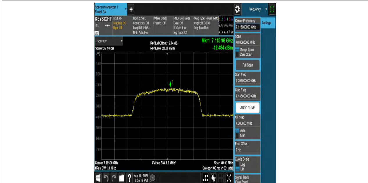
11AX20MIMO-Ant2-7115-PASS
