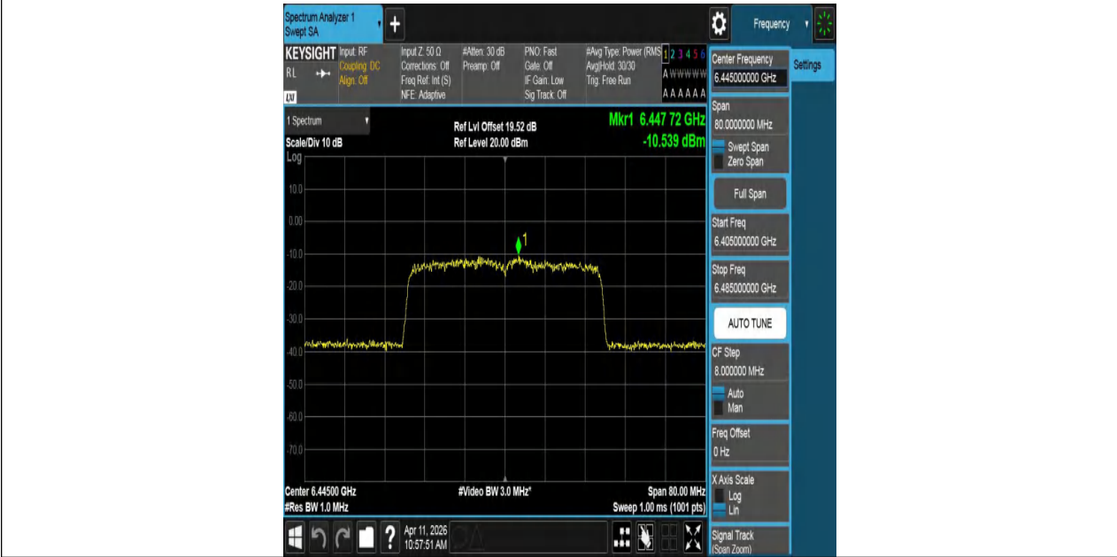
11BE40MIMO-Ant1-6445-PASS
