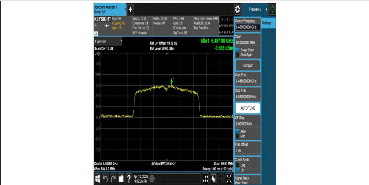
11AX40MIMO-Ant2-6485-PASS
