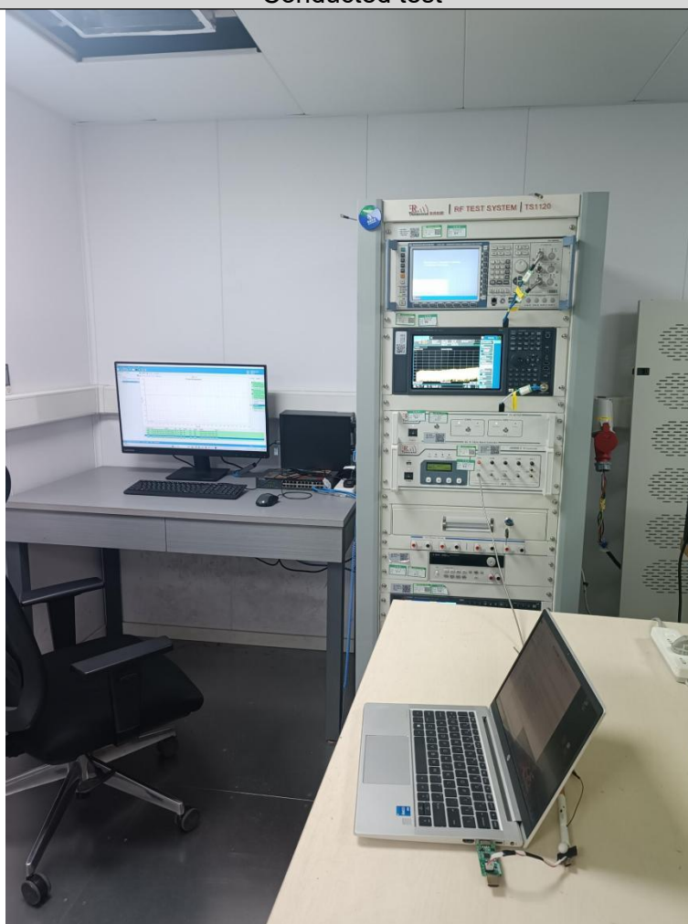
Conducted test
