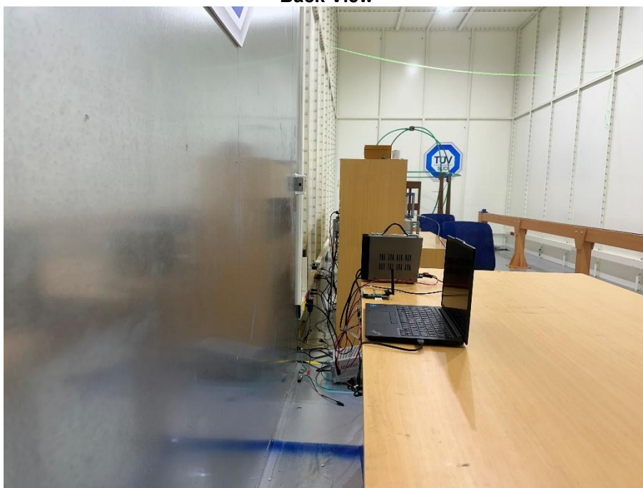
Set-up for Conduction Emissions Back View
