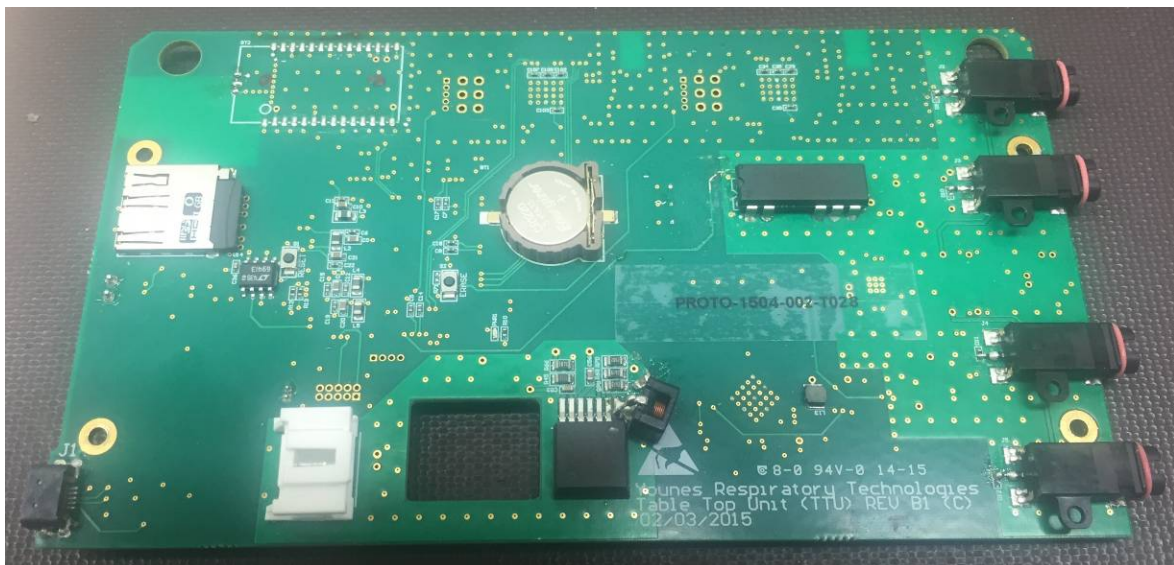
Figure 2 – EUT Internal Photo Back
