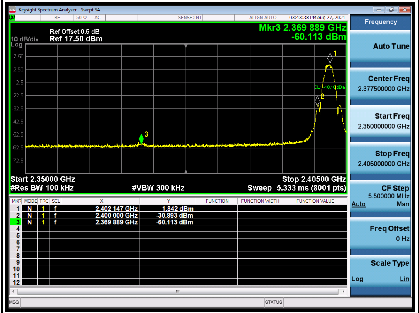
Mode2/CH00/2402MHz
