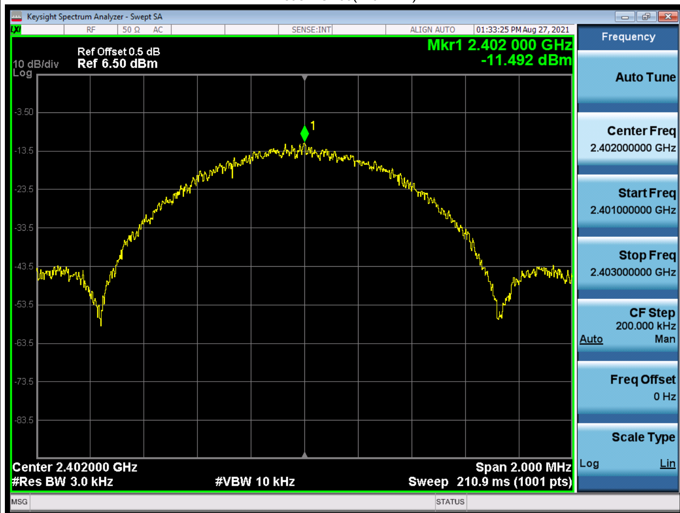
Mode 1 CH00(2402MHz)
