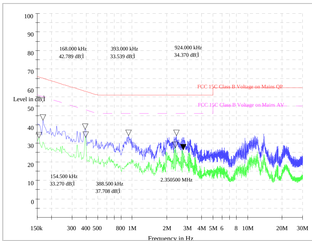
Voltage Test
