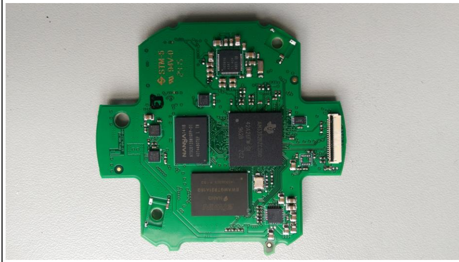
EUT PCB 1 Front
