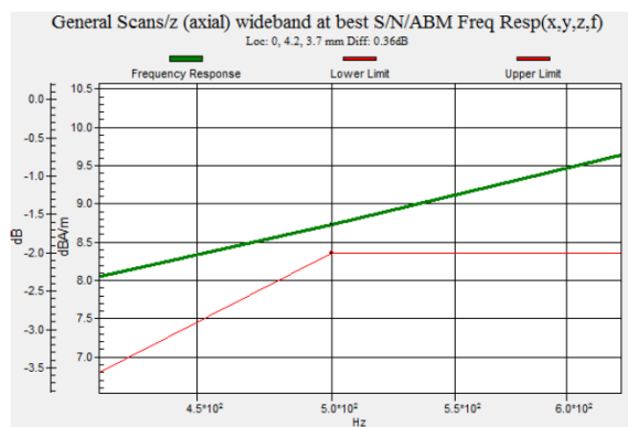
Fig 7.4 GSM1900 Ch661
