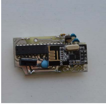
Figure 1 Sensor Inside Top
