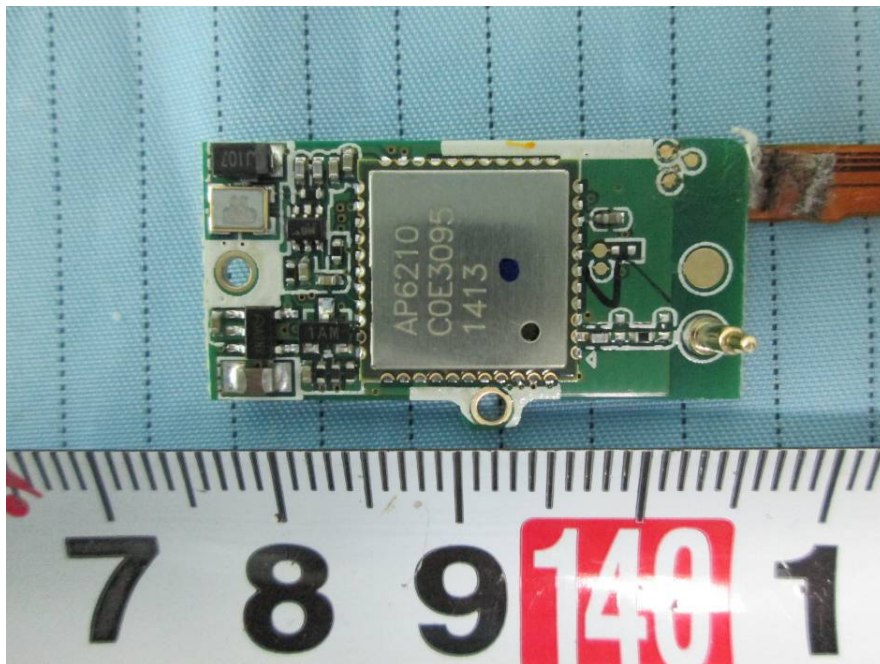
EUT – Main Board 3 Bottom Shielding off View 1
