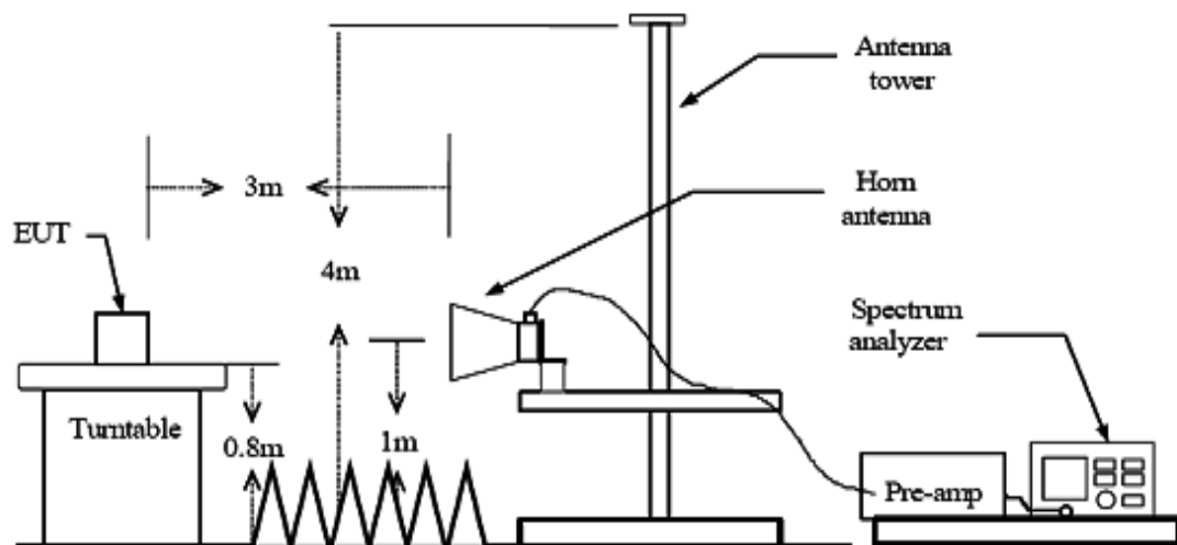
Above 1GHz
