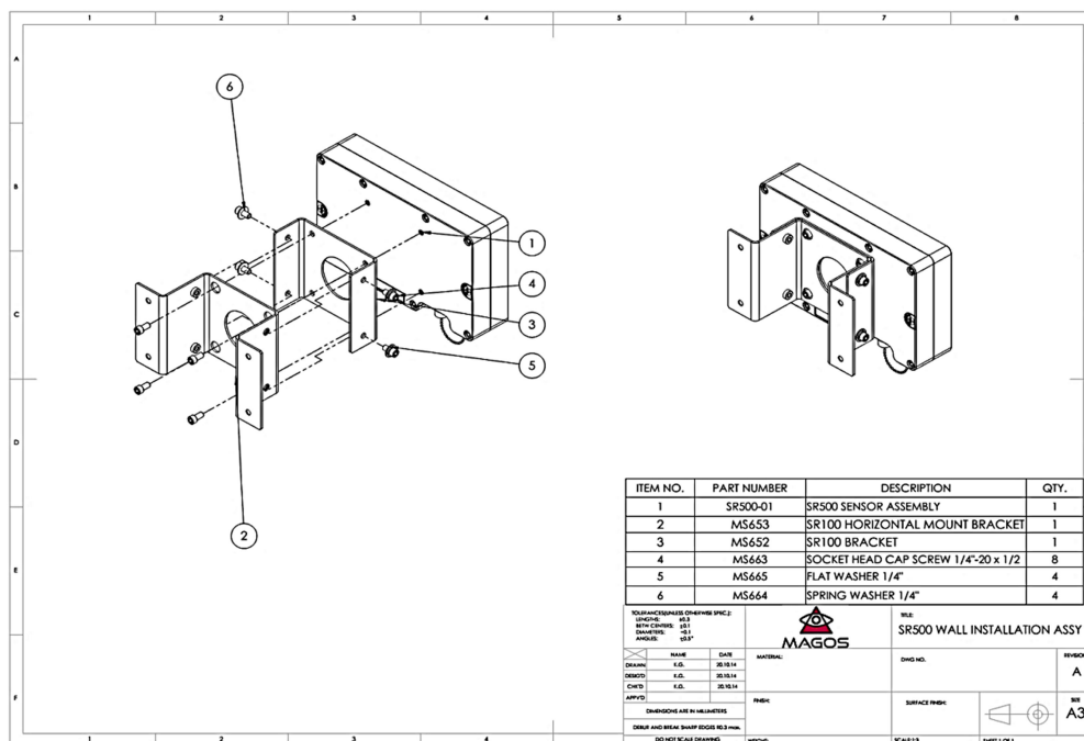
Figure 4: SR Wall Installation
