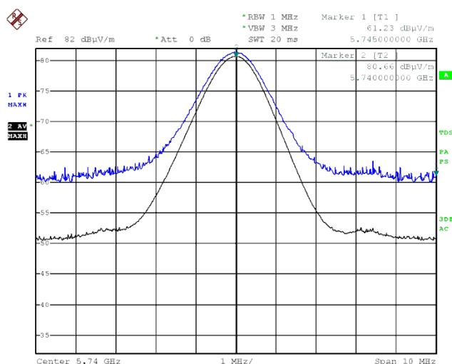
Figure 12. Field Strength of Fundamental. HORIZONTAL – Low
