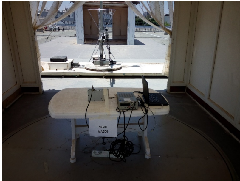
Figure 4. Spurious Radiated Emission Test
