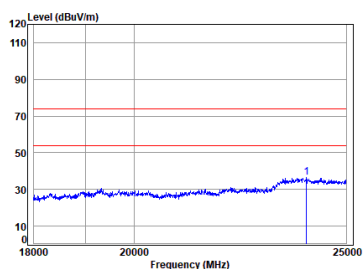
BT_TX_CH_M_Vertical
