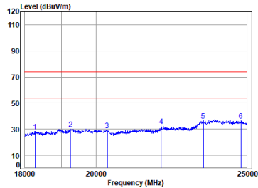
BLE_2M_TX_CH_00_Horizontal
