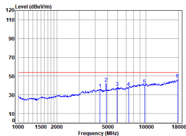
BLE_1M_TX_CH_19_Horizontal-Avg
