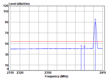
BLE_1M_TX_CH_00_Vertical-AVG
