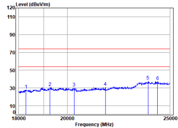
BLE_2M_TX_CH_00_Vertical
