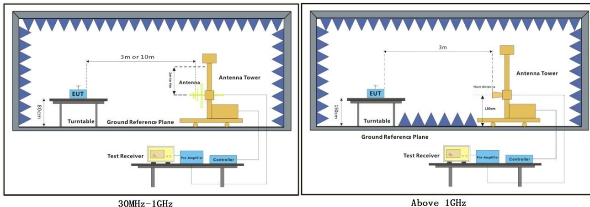
30MHz-1GHz
