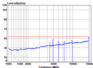
BLE_1M_TX_CH_19_Horizontal-Avg
