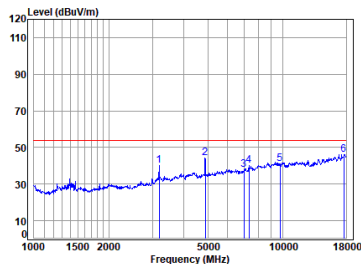
BLE_1M_TX_CH_19_Vertical-Avg
