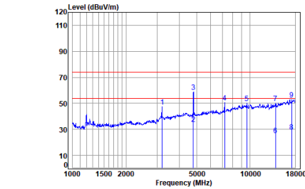
BT_DH5_TX_CH_00_Horizontal
