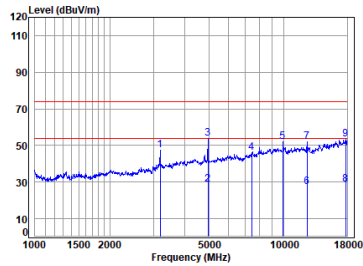
BT_DH5_TX_CH_78_Horizontal
