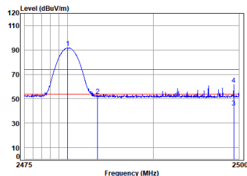
BT_2DH5_TX_CH_78_Vertical
