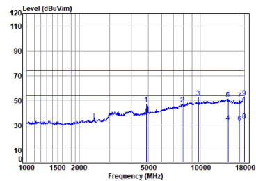
BT_2DH5_TX_CH_39_Vertical
