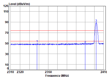
BT_2DH5_TX_CH_00_Vertical
