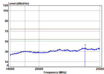
BT_2DH5_TX_CH_39_Vertical
