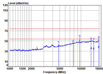
BT_2DH5_TX_CH_00_Horizontal
