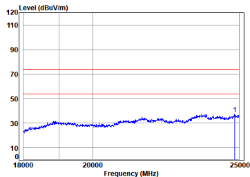
BT_2DH5_TX_CH_78_Horizontal
