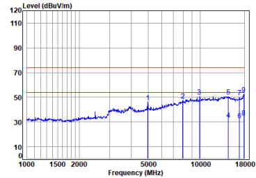
BT_2DH5_TX_CH_78_Vertical
