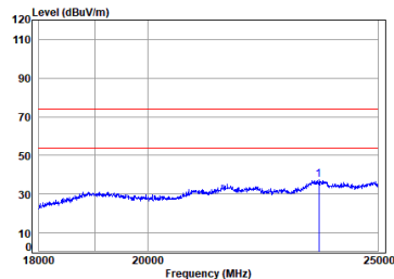
BT_2DH5_TX_CH_78_Vertical
