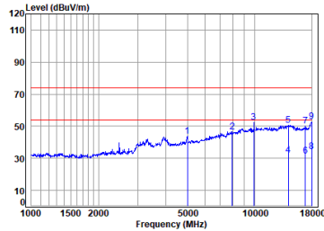
BT_2DH5_TX_CH_78_Horizontal
