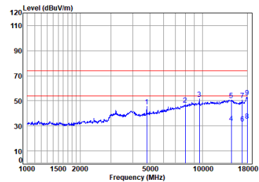
BT_2DH5_TX_CH_00_Vertical
