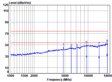
BT_DH5_TX_CH_00_Horizontal
