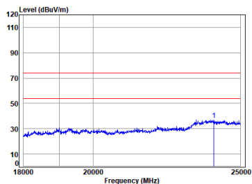
BT_DH5_TX_CH_39_Vertical
