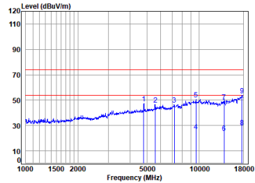
BT_DH5_TX_CH_00_Vertical
