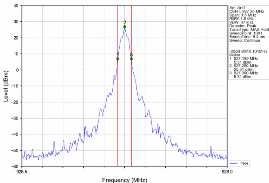
TX_HCH_927.25MHz_Ant1_NTNV
