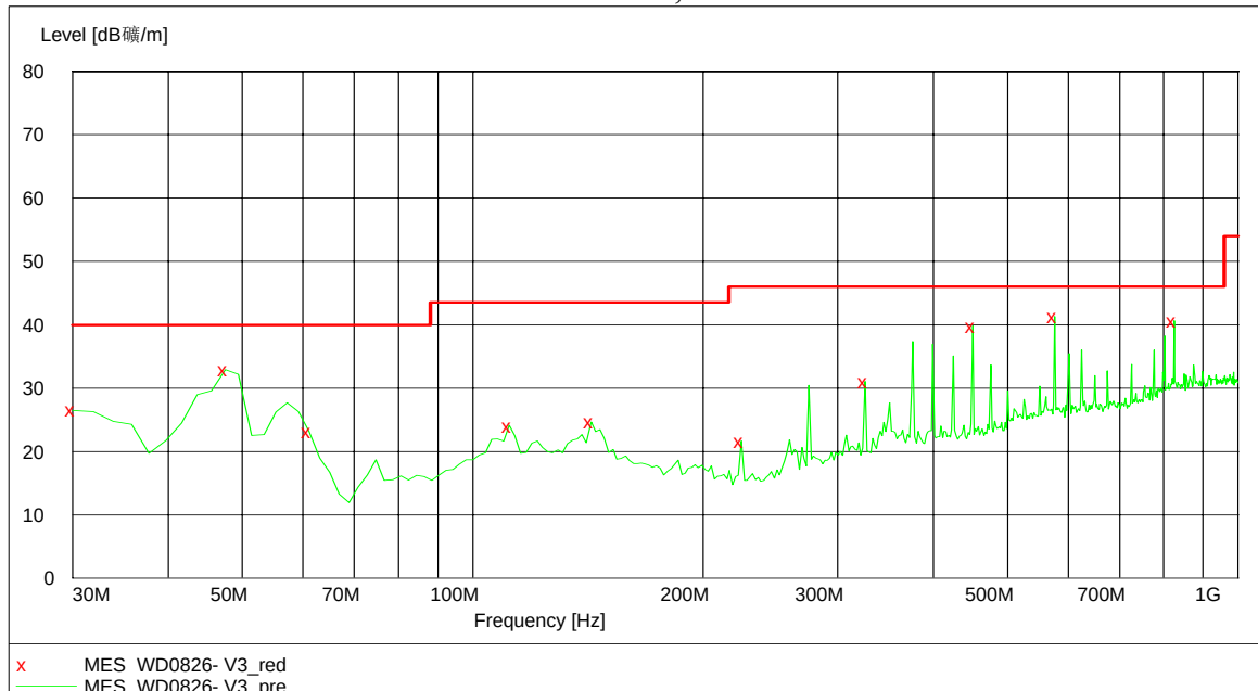
30MHz~1GHz, Vertical
