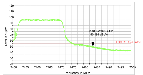
802.11n HT20 -Channel 11 Average
