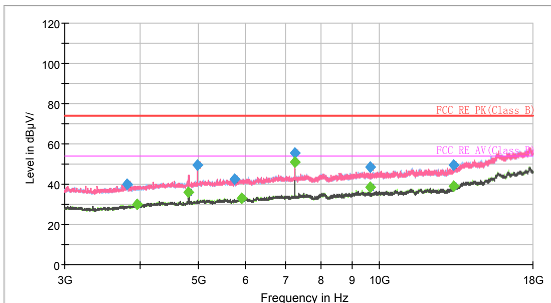
Radiates Emission from 3GHz to 18GHz
