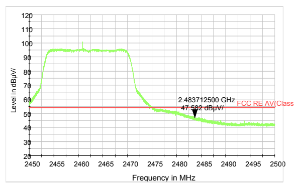
802.11g-Channel 11 Average
