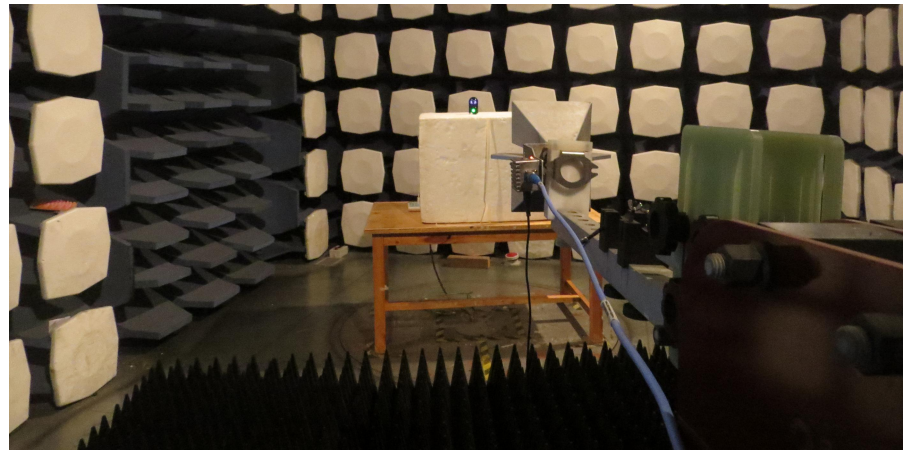
Picture 2 Radiated Emission Test Setup
