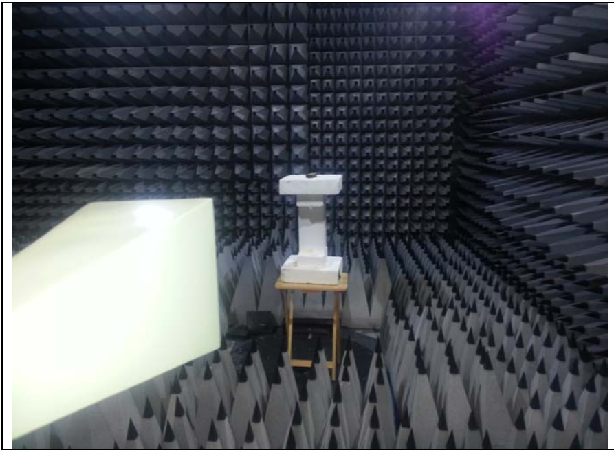
Fig 3 Test setup 18GHz -26.5 GHz Rad Emissions
