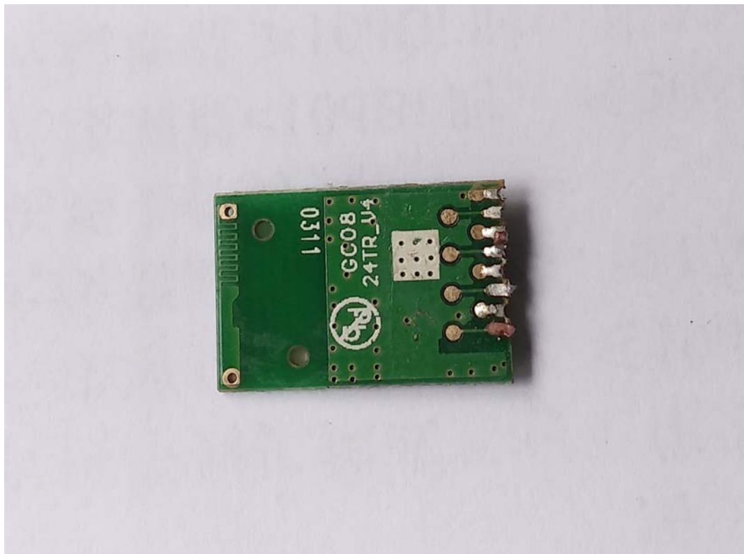
FIGURE 8 REMOTE CONTROLLER (M/N: SK007-1) RF MODULE (SOLDERED SIDE)
