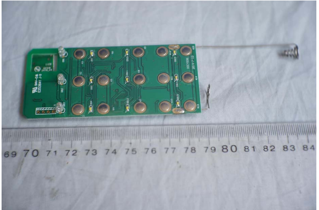
FIGURE 5 REMOTE CONTROLLER (M/N: SK007-1) MAIN BOARD (SOLDERED SIDE)
