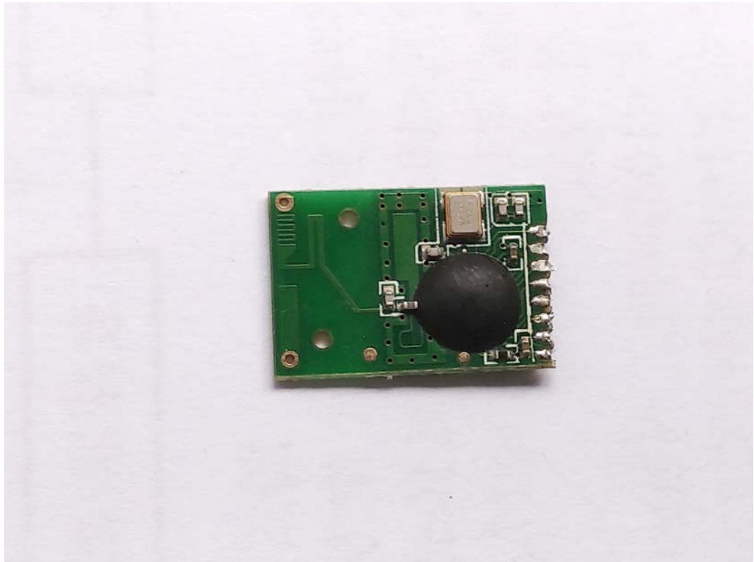
FIGURE 7 REMOTE CONTROLLER (M/N: SK007-1) RF MODULE (COMPONENT SIDE)
