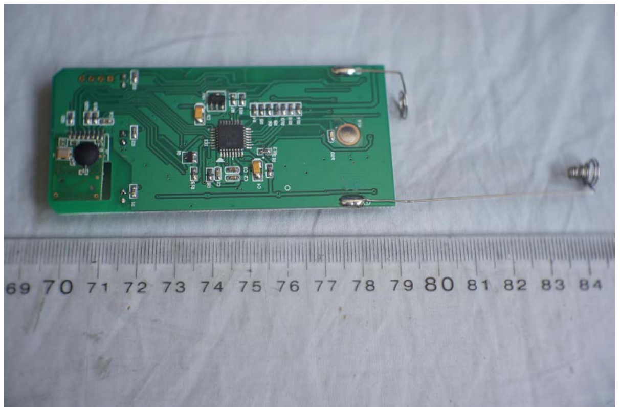
FIGURE 4 REMOTE CONTROLLER (M/N: SK007-1) MAIN BOARD (COMPONENT SIDE)
