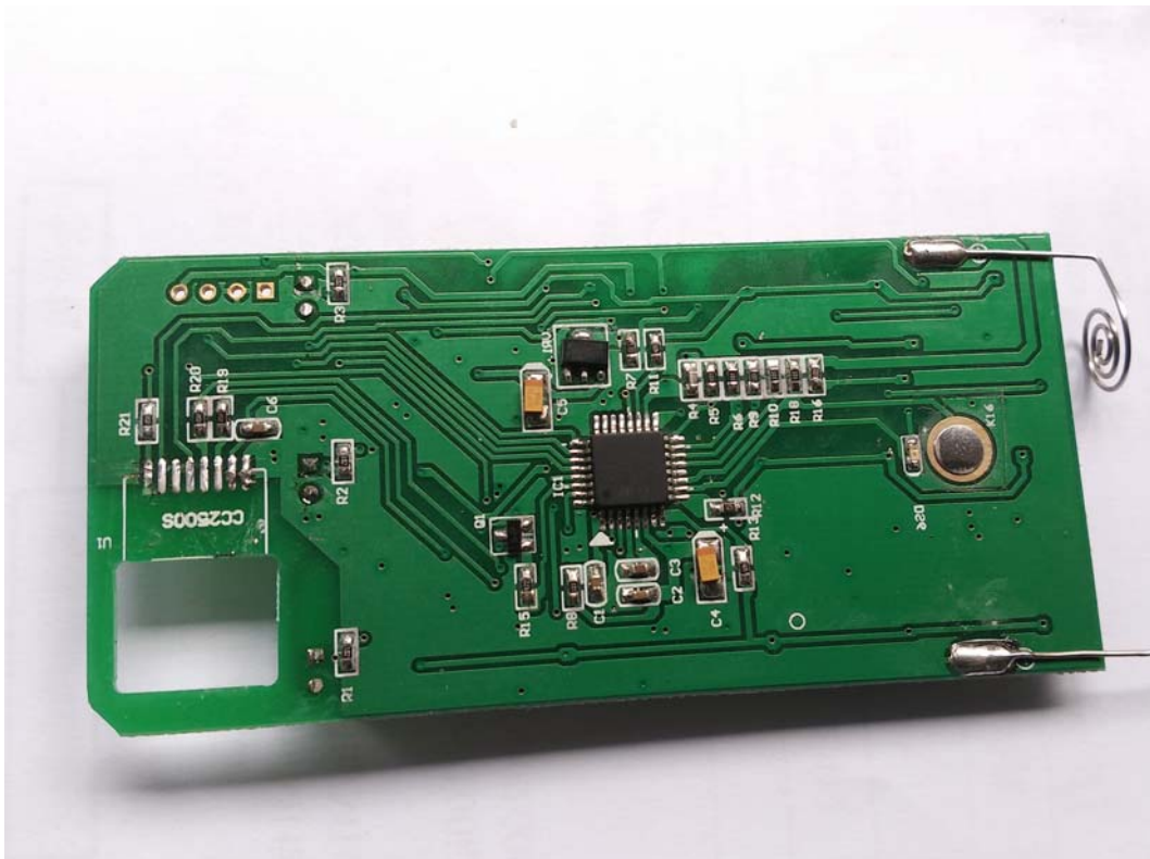
FIGURE 6 REMOTE CONTROLLER (M/N: SK007-1) MAIN BOARD (RF MODULE REMOVED )
