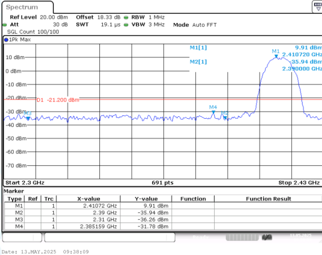
11B-CDD-Ant1-2412-PASS
