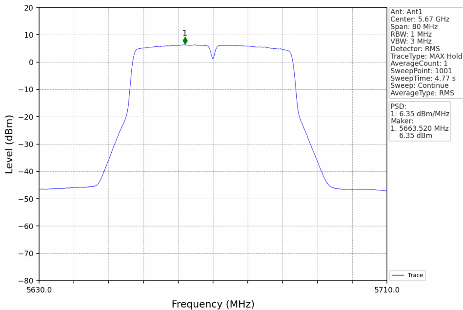
802.11n(HT40)_HCH_5670MHz_Ant1_NTNV
