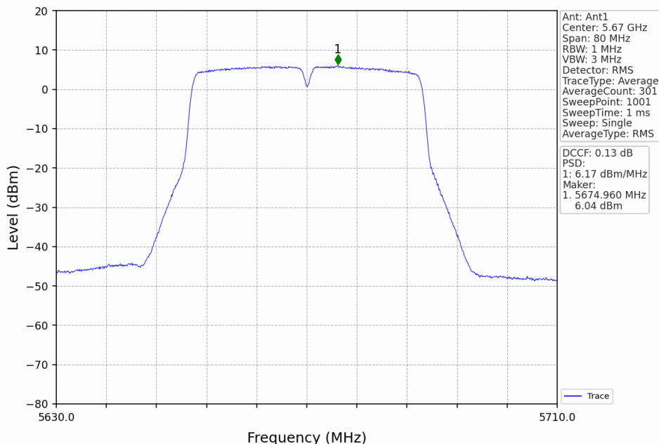
802.11ac(VHT40)_HCH_5670MHz_Ant1_NTNV
