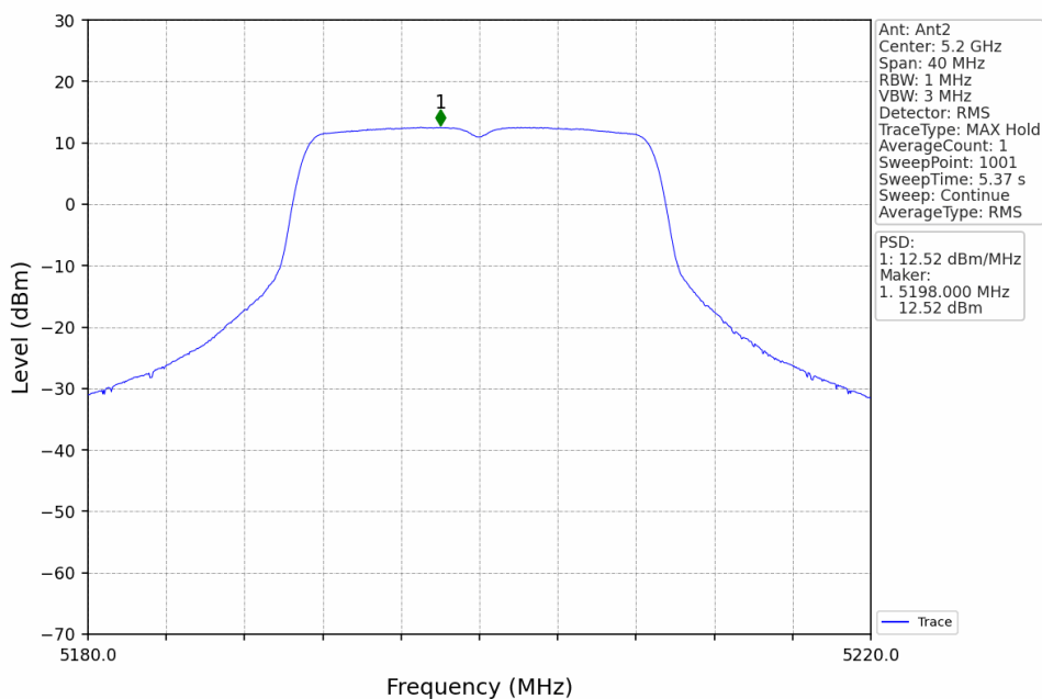
802.11ac(VHT20)_MCH_5200MHz_MIMO_NTNV
