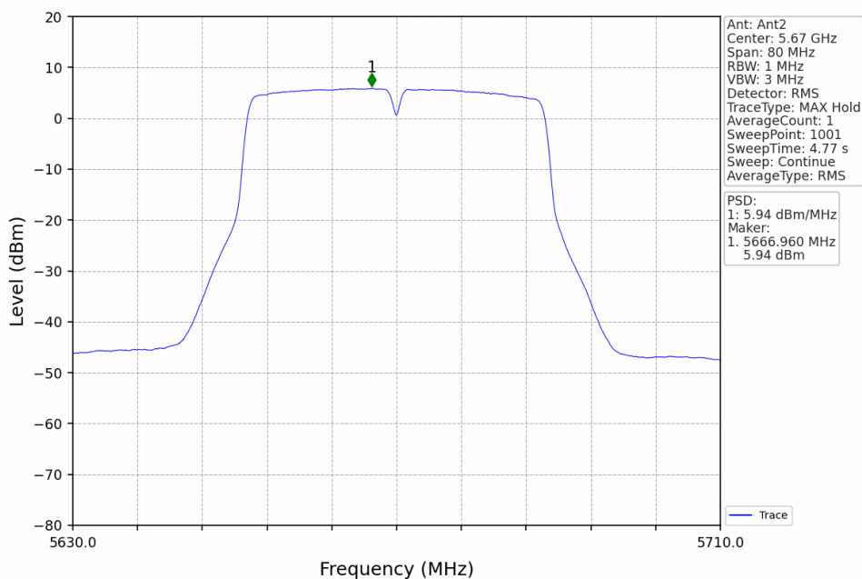
802.11n(HT40)_HCH_5670MHz_MIMO_NTNV
