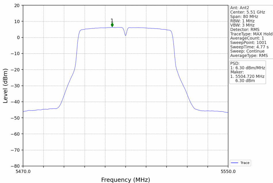
802.11n(HT40)_LCH_5510MHz_MIMO_NTNV
