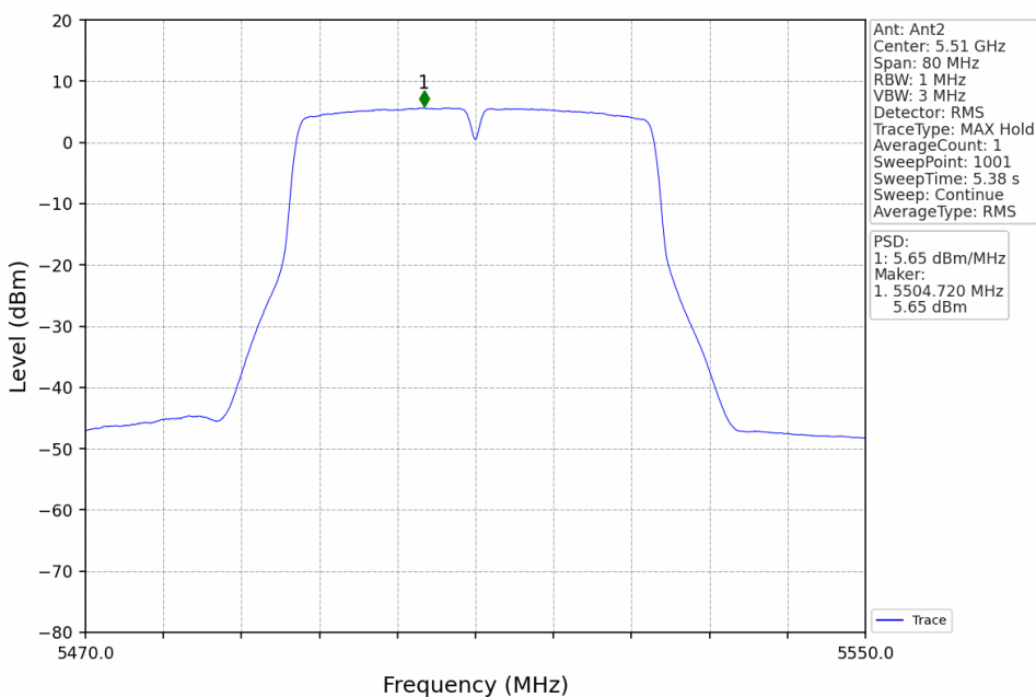
802.11ac(VHT40)_LCH_5510MHz_MIMO_NTNV
