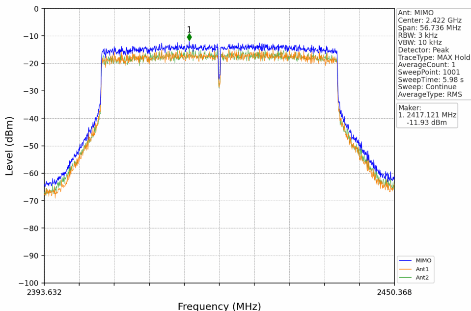
802.11ax(HEW40)_LCH_2422MHz_RU484_Left_MIMO_NTNV
