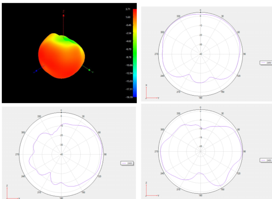
2G-1-2450MHz
