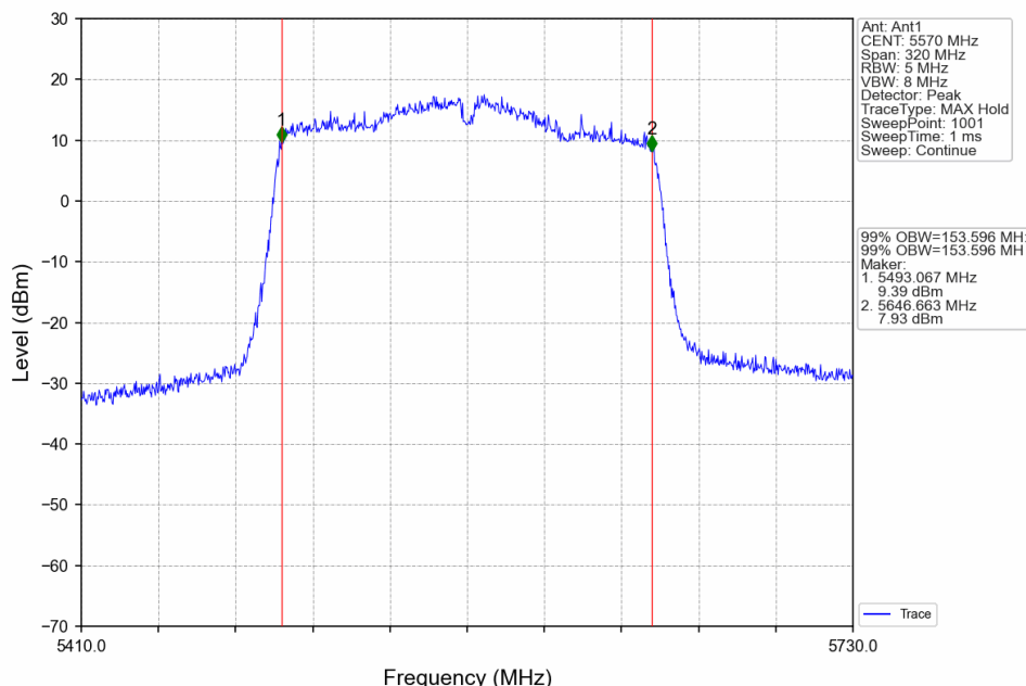
802.11ac(VHT160)_MCH_5570MHz_Ant1_NTNV
