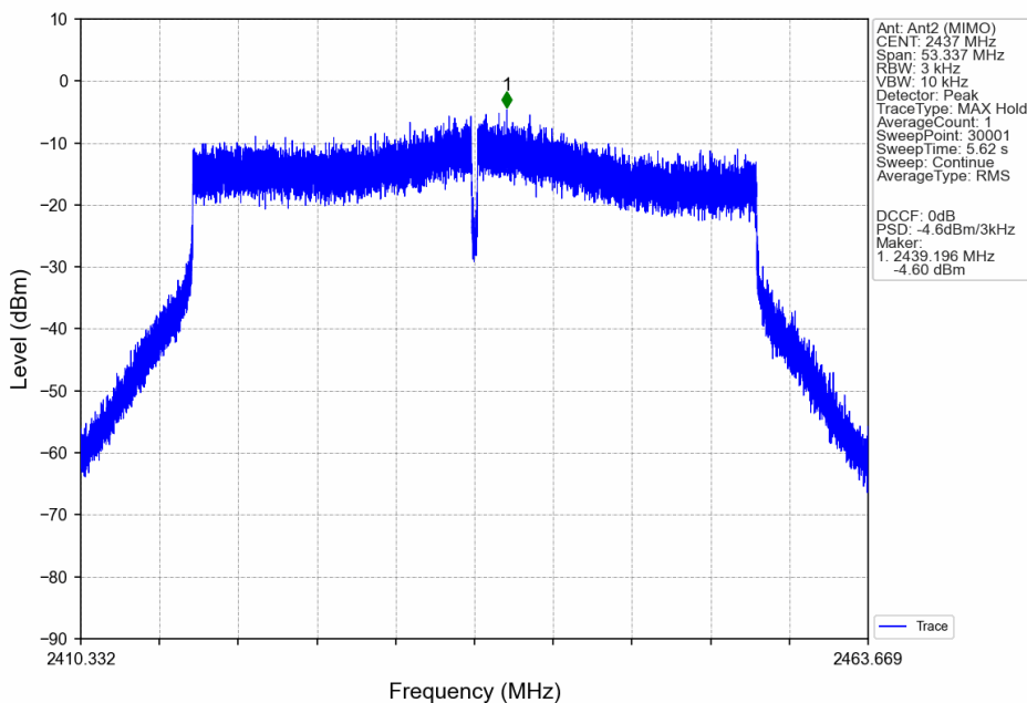
802.11ax(HEW40)_MCH_2437MHz_SU_/_Ant2 (MIMO)_NTNV
