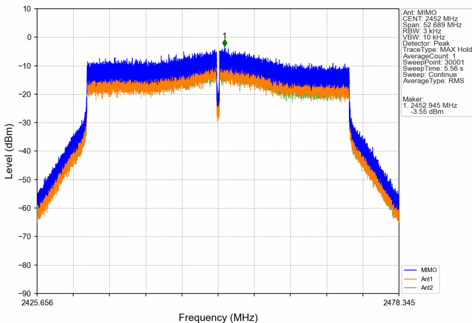
802.11be(EHT40)_HCH_2452MHz_SU_/_MIMO_NTNV
