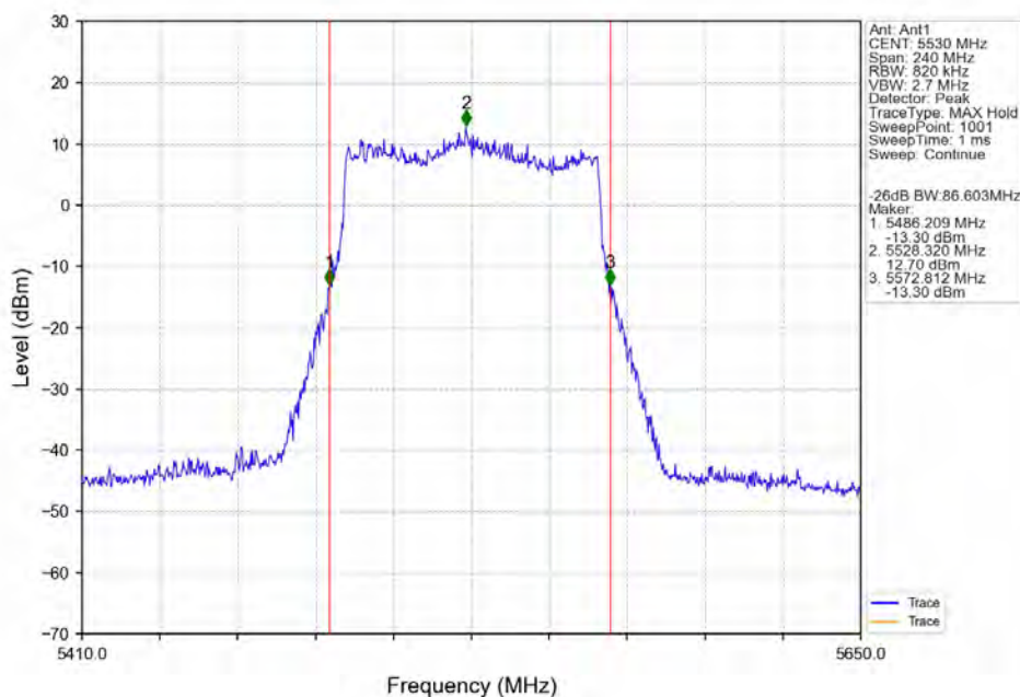
802.11ax(HEW80)_LCH_5530MHz_SU_/_Ant1_NTNV
