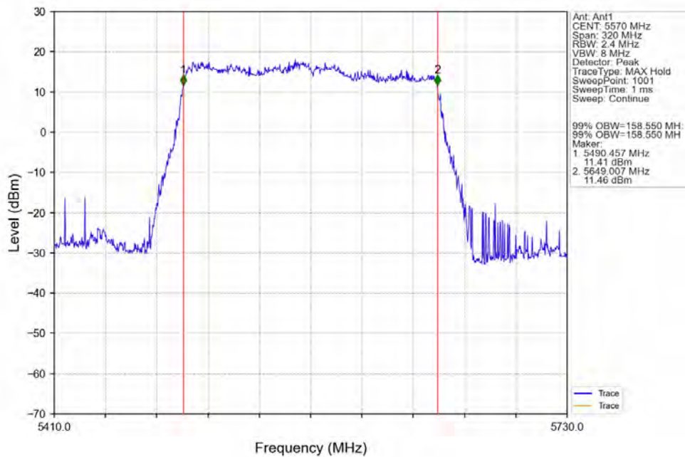
802.11ax(HEW160)_MCH_5570MHz_SU_/_Ant1_NTNV
