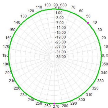
H面-THET=90
