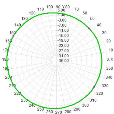
H面-THET=90
