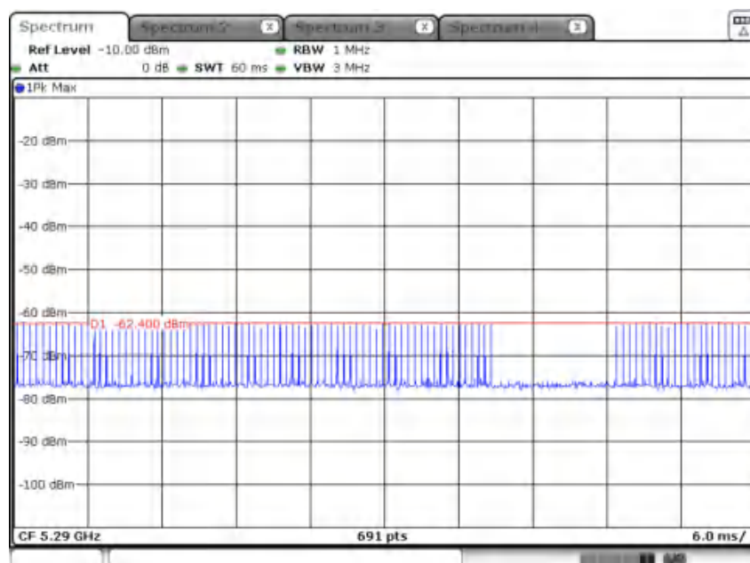
Radar Type 1 Calibration Plot (5290MHz)
