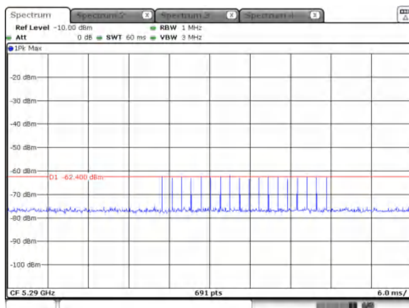
Radar Type 0 Calibration Plot (5290MHz)
